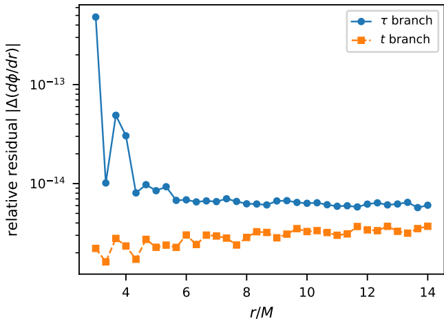
Thakurta-Kerr, static limit A = 1 : Hamilton flow vs closed-form equatorial Kerr ( s = 0.9, E = 1.2, J = 1.3 )
