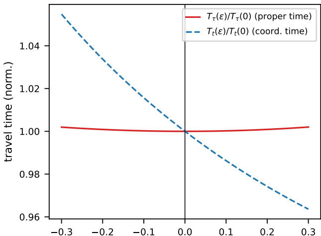
t -brachistochrone: perturbing r(\varphi) at fixed endpoints
