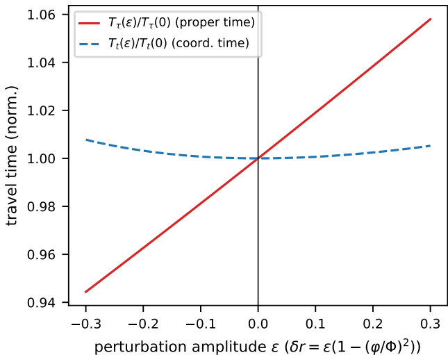
t -brachistochrone: perturbing r(\varphi) at fixed endpoints
