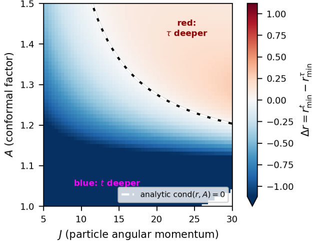
Conformal plunge inversion (Thakurta-Kerr, s = 0.9 , \hat{E} = 1.2 ): \Delta r changes sign; inversion curve analytic = numeric, REACHABLE ( A_{\text{inv}} < A_{\text{freeze}} )
