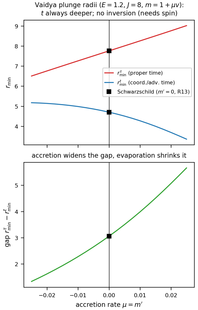
FIG. 8. Plunge radii r_{\min}^{t,\tau} and gap vs \mu = m' ; t deeper, accretion widens the gap.
