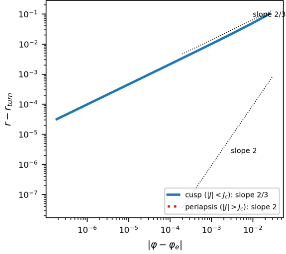
FIG. 12. Reflection at the ergosphere: cusp ( |J| < J_c ), smooth crossing to r_+ in Doran coordinates ( |J| = J_c ), smooth periapsis ( |J| > J_c ); power law 2/3 vs 2 .
