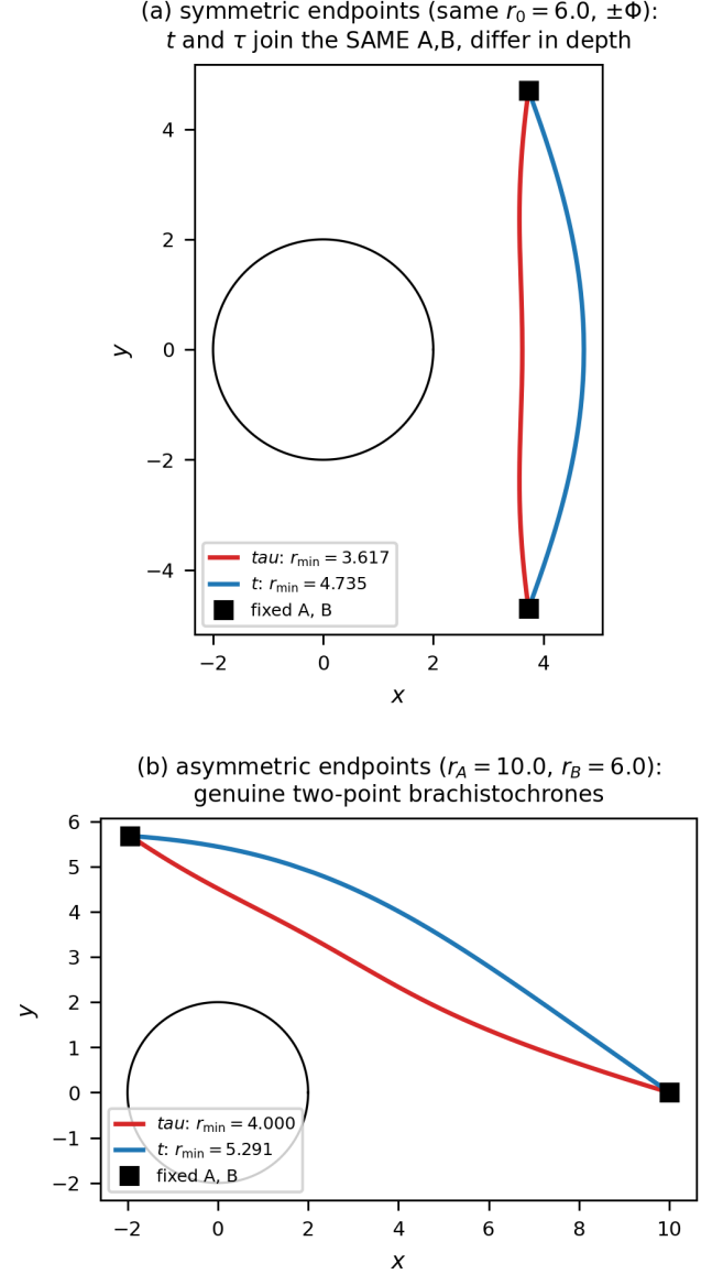
FIG. 15. Fixed-endpoint t and \tau brachistochrones (Schwarzschild, E = 1.2 ): symmetric (top) and asymmetric (bottom) endpoints. Both branches join the same A, B ; the \tau -branch dips deeper.
