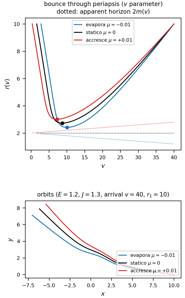
FIG. 6. Bounce through periapsis in the v -parametrization: the Euler–Lagrange flow is regular at r' = 0 and integrates through the turning point, reaching r_{\min} exactly where the r -parametrization diverges.
