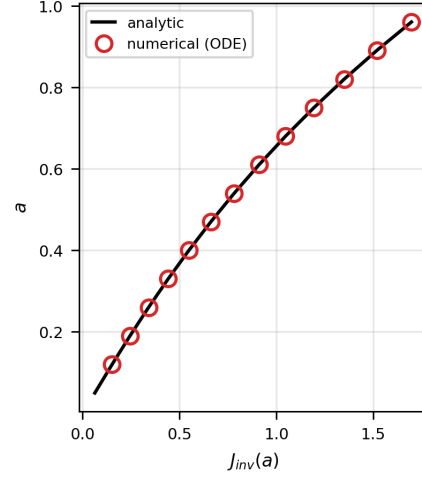
FIG. 13. Rotational inversion in the (a, J) plane; ODE locus vs analytic \rho(r_*)^2 = H_{t0}/H_{\tau0} .
