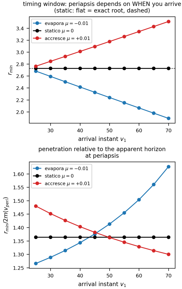
FIG. 7. Timing window: r_{\min} depends on the arrival epoch v_1 . The orbit-horizon race has opposite winners in absolute ( r_{\min} ) and relative ( r_{\min}/2m ) terms for accretion vs evaporation.
