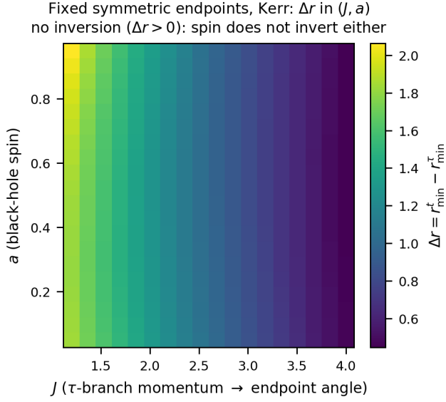
FIG. 16. Spin scan at fixed symmetric endpoints (Kerr, Hamiltonian flow): \Delta r in the (J, a) plane stays positive everywhere—spin does not invert once the endpoints are pinned. The gradient is set by the endpoint angle ( J ), not by a .
