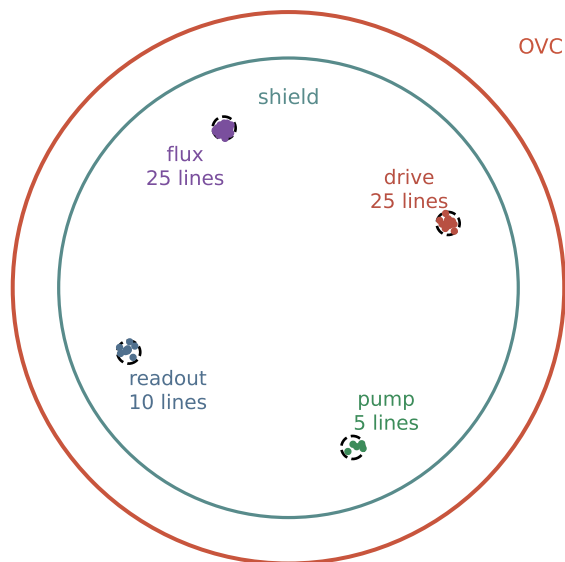
(a) 65 coaxial lines in four functional families
