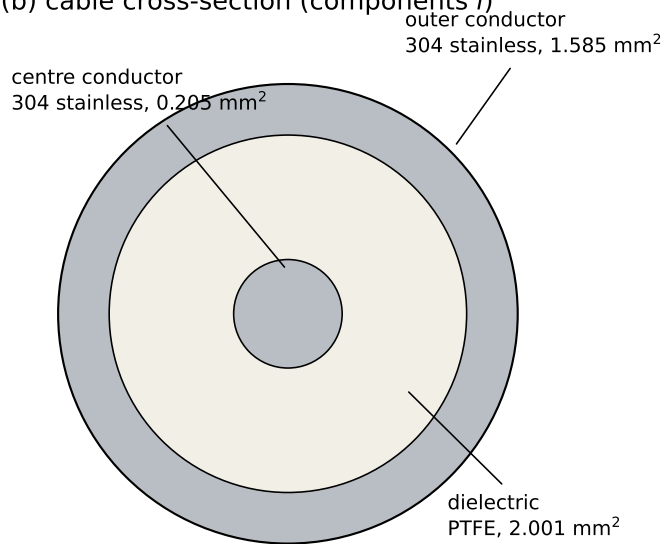
(b) cable cross-section (components i )
