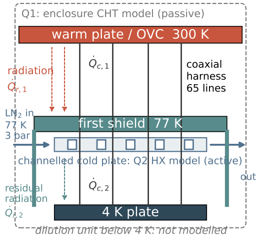
(c) route N 2 : liquid nitrogen 77 K in, 3 bar
