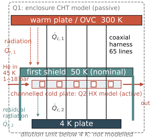
(b) route He: circulated gas 45 K in, 1--18 bar
