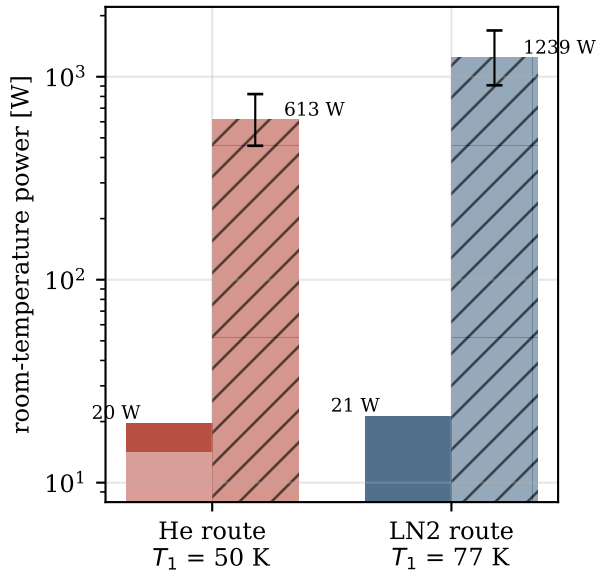
(b) MLI-equivalent shield ( \epsilon = 0.003 )
