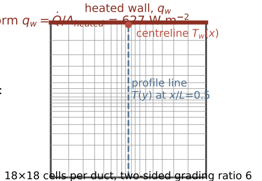
(b) duct cross-section: mesh and sampling lines
