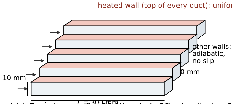
(a) cold-plate heat-exchanger domain
