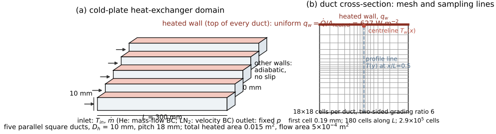
Figure 5: Cold-plate heat-exchanger model: (a) the five heated square ducts with boundary conditions and dimensions; (b) the graded duct cross-section with the two sampling lines used for the wall-temperature profiles.
