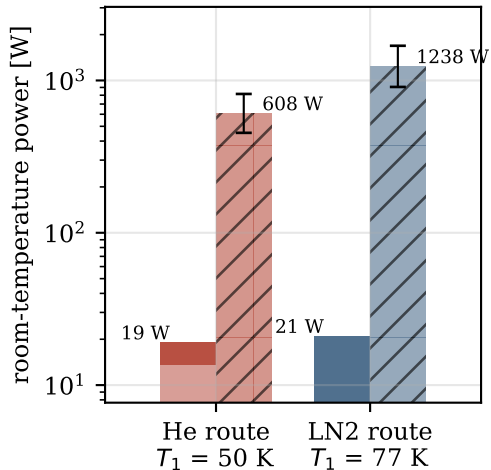
(b) MLI-equivalent shield ( \epsilon = 0.003 )
