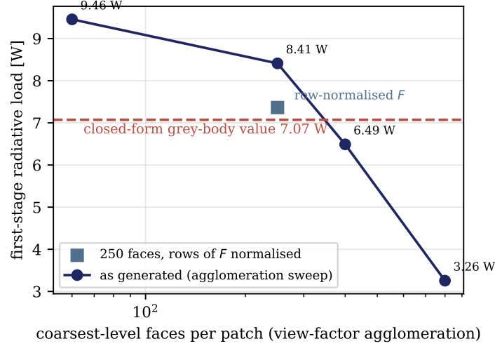
Figure 6: First-stage radiative load (300 \rightarrow 50 K) against the view-factor agglomeration level with the matrix as generated (circles) and with its rows normalised to unity at the production level (square), compared with the closed-form grey-body value. The monotonic collapse under refinement is a closure artefact amplified by the low emissivities.
