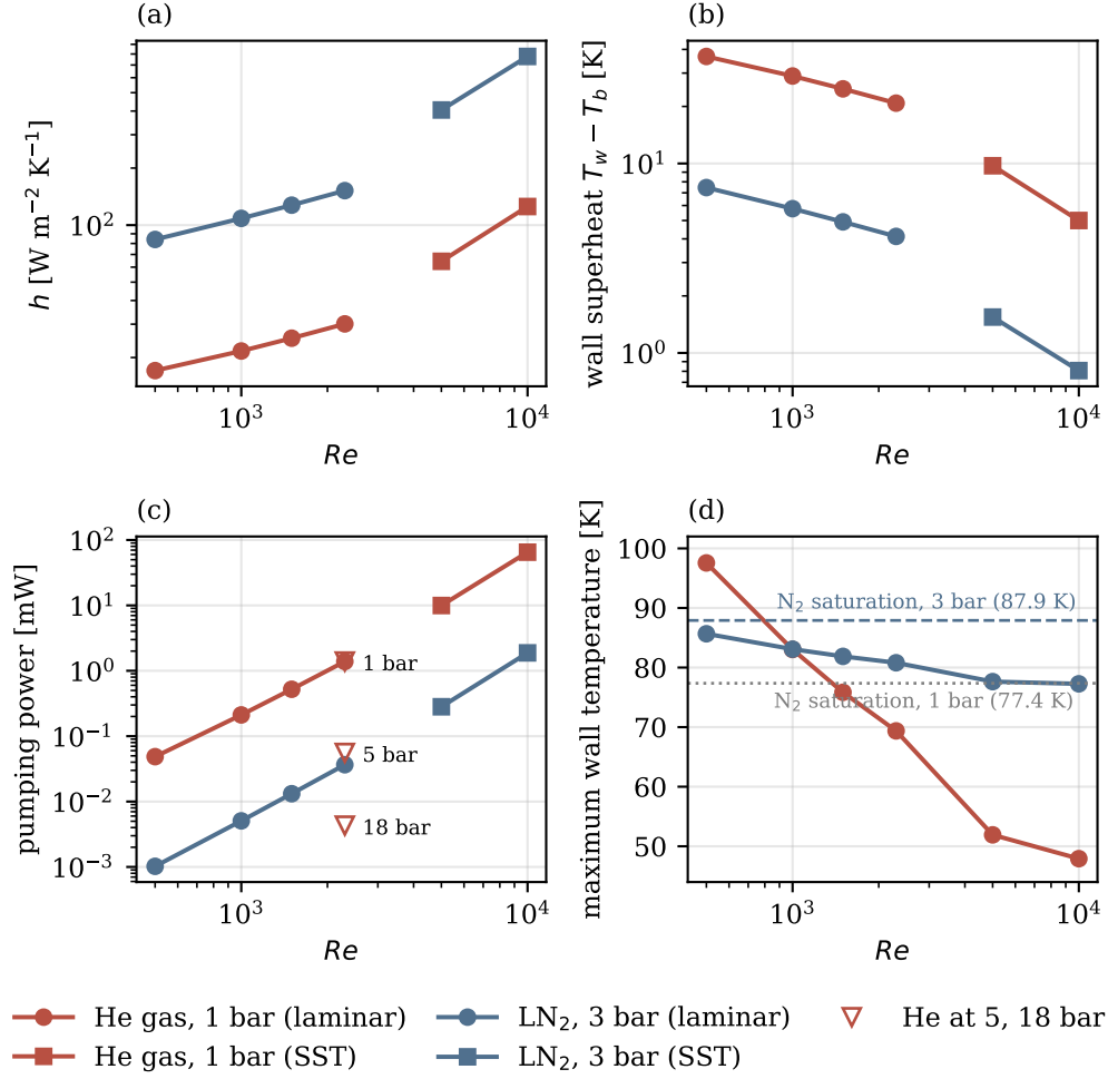
Figure 9: Operating maps at 9.4 W duty: (a) heat-transfer coefficient, (b) wall superheat, (c) pumping power with the helium pressure series at Re = 2300 , and (d) maximum wall temperature with the nitrogen saturation temperatures at 1 and 3 bar. Circles: laminar; squares: k-\omega SST.
