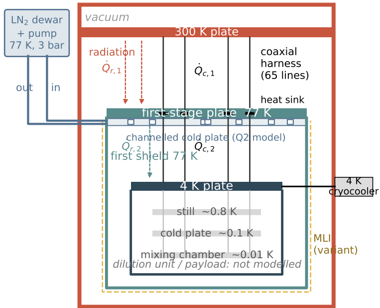
(b) liquid-nitrogen route, first stage 77 K
