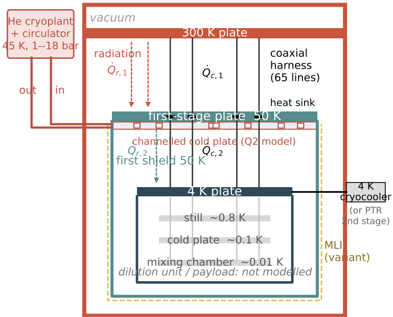
(a) helium-gas route, first stage 50 K (nominal)
