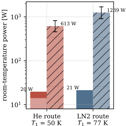
(b) MLI-equivalent shield ( \epsilon = 0.003 )
