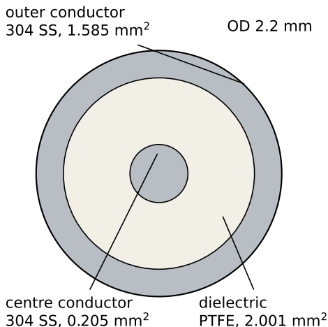
(b) UT-085 cable cross-section
