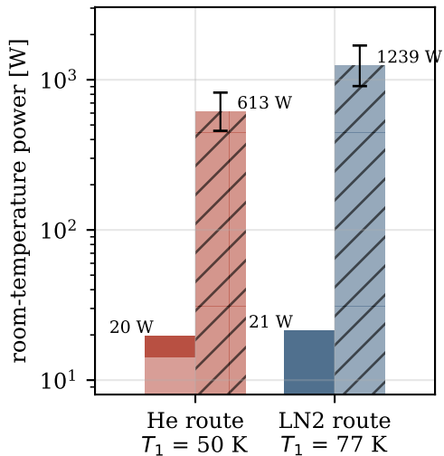
(b) MLI-equivalent shield ( \epsilon = 0.003 )
