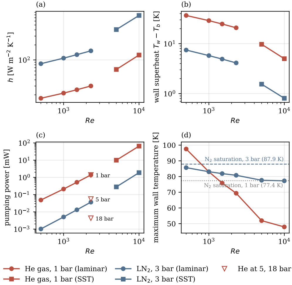
Figure 9: Operating maps at 9.4 W duty: (a) heat-transfer coefficient, (b) wall superheat, (c) pumping power with the helium pressure series at Re = 2300 , and (d) maximum wall temperature with the nitrogen saturation temperatures at 1 and 3 bar. Circles: laminar; squares: k-\omega SST.
