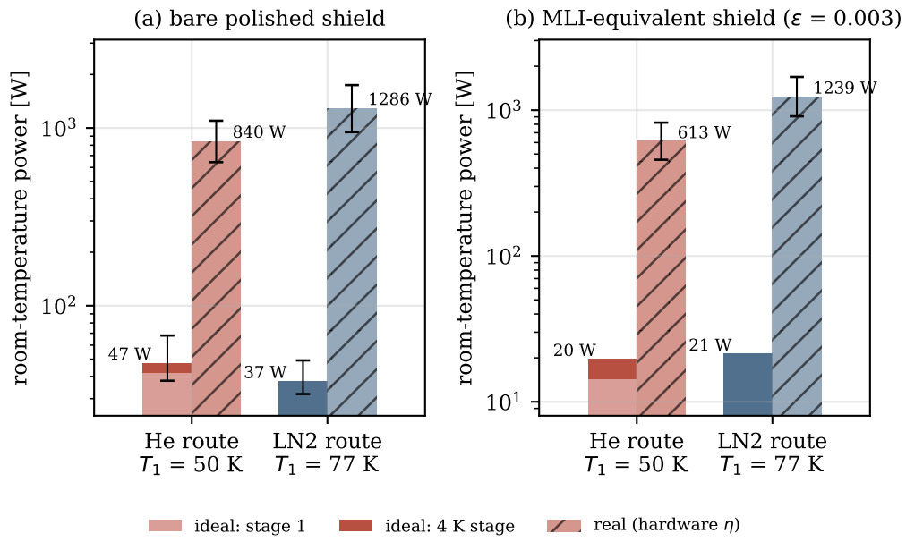
Figure 12: Room-temperature power of the two routes for (a) the bare polished shield and (b) the MLI-equivalent shield: ideal Carnot multipliers split by stage (solid) and hardware efficiencies (hatched), with emissivity and efficiency ranges as error bars.
