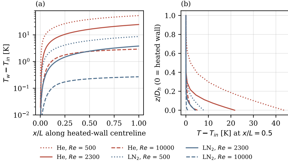
Figure 10: (a) Heated-wall centreline temperature rise above the inlet and (b) cross-channel temperature profile at x/L = 0.5 for both fluids at Re = 500 , 2300 and 10^4 .
