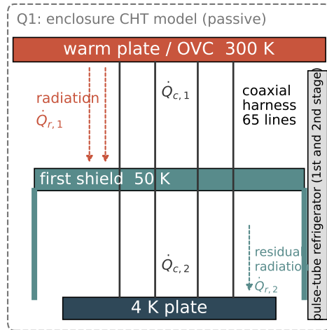
(a) reference: PTR first stage 40--50 K, conductive
