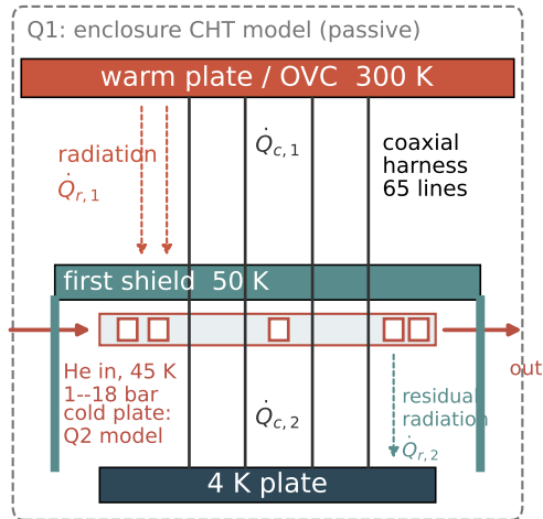
(b) route He: circulated gas 50 K nominal; 45 K in, 1--18 bar
