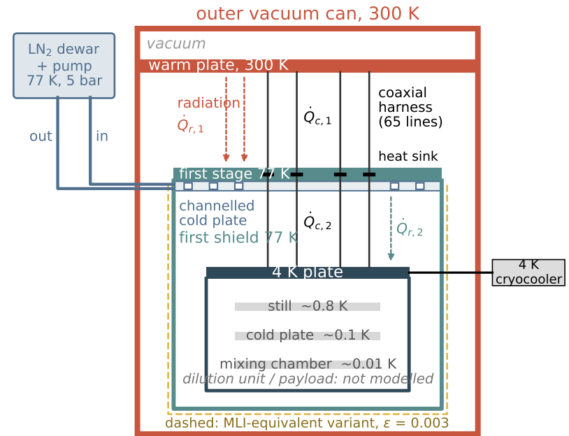
(b) liquid-nitrogen route, first stage 77 K
