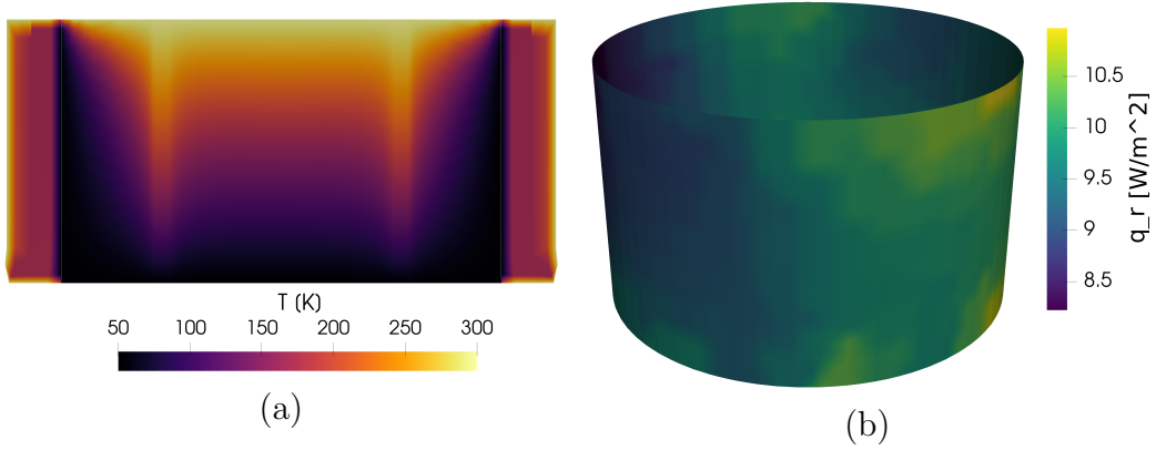
Figure 7: (a) Mid-plane temperature and (b) shield radiative-flux map of the 300 \rightarrow 50 K case.
