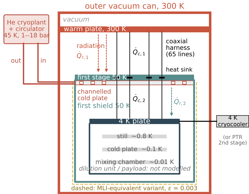
(a) helium-gas route, first stage 50 K (nominal)
