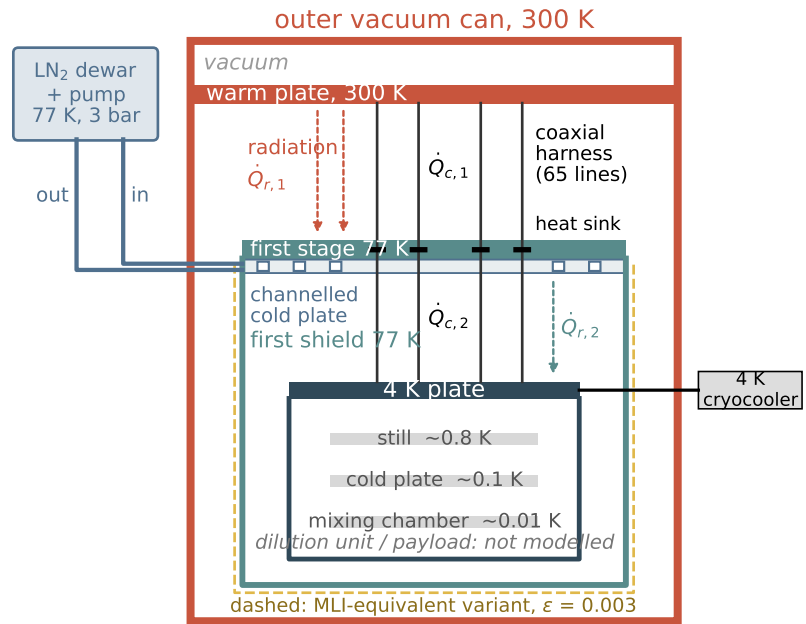
(b) liquid-nitrogen route, first stage 77 K
