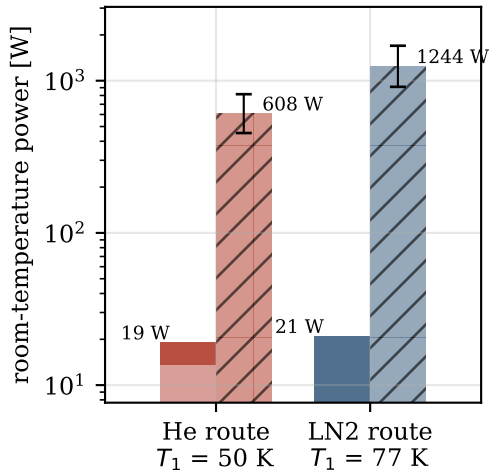
(b) MLI-equivalent shield ( \varepsilon = 0.003 )
