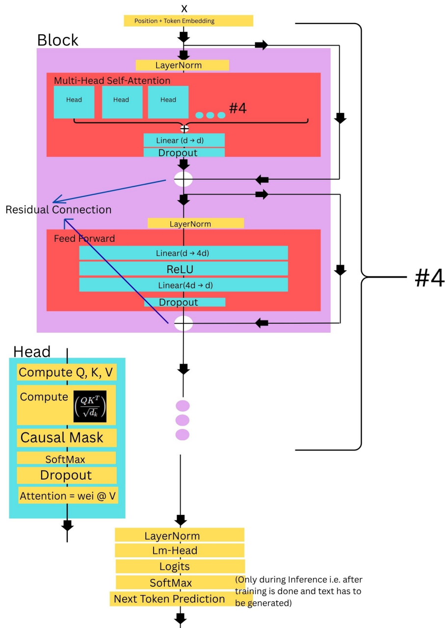
Figure 1: Architecture of the implemented Transformer language model.
