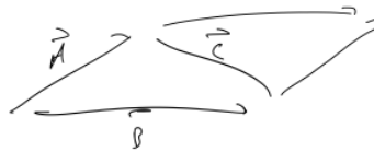
Figure 14: Law of cosines
