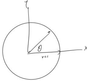
Figure 17: Circular motion on the unit circle.
