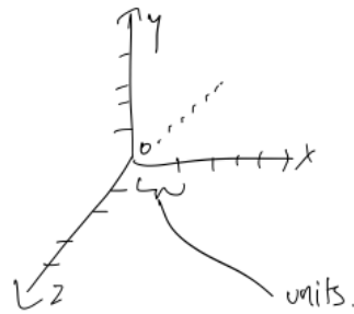
Figure 10: Cartesian coordinate system.
