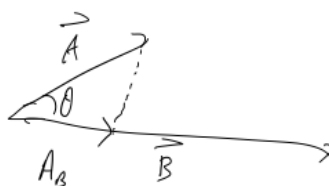
Figure 13: Dot product visually
