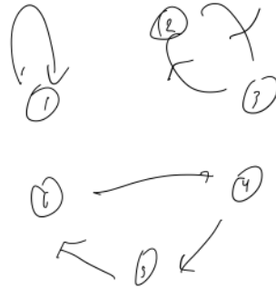
Figure 6: Dice laws of motion.
