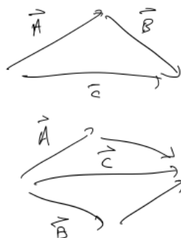
Figure 12: Adding vectors.
