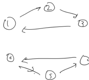
Figure 5: Dice laws of motion.
