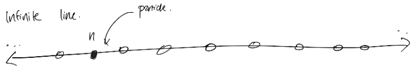
Figure 7: An infinite number of states.
