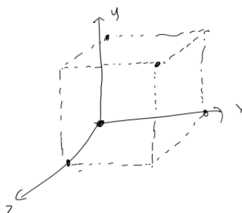
Figure 11: Coordinates.
