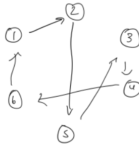
Figure 4: Dice laws of motion.
