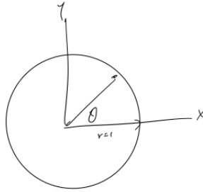
Figure 17: Circular motion on the unit circle.
