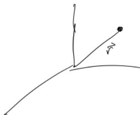
Figure 15: Particle.
