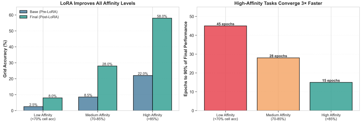
FIGURE 4. LoRA Fine-Tuning Efficiency by Affinity Level. Left panel: High-affinity tasks (base cell accuracy > 85%) achieve substantially higher final grid accuracy (58.0%) compared to low-affinity tasks (< 70%: 8.0%). Right panel: Convergence speed correlates with affinity—high-affinity tasks reach 90% of final performance in 15 epochs vs. 45 epochs for low-affinity tasks. Demonstrates that architectural mismatch creates efficiency ceilings independent of data quantity.
