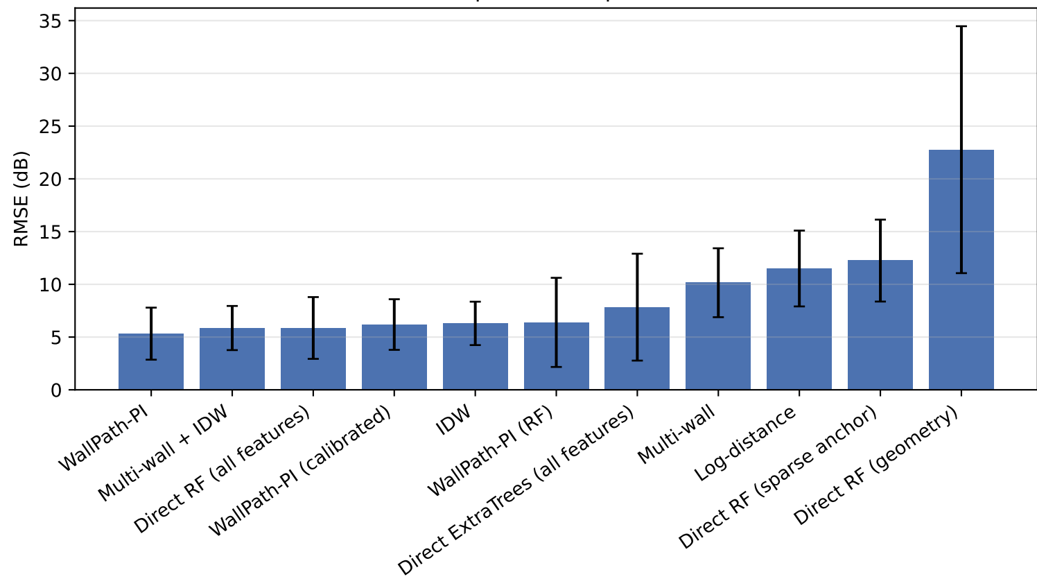
Method comparison at sparse rate 0.01
