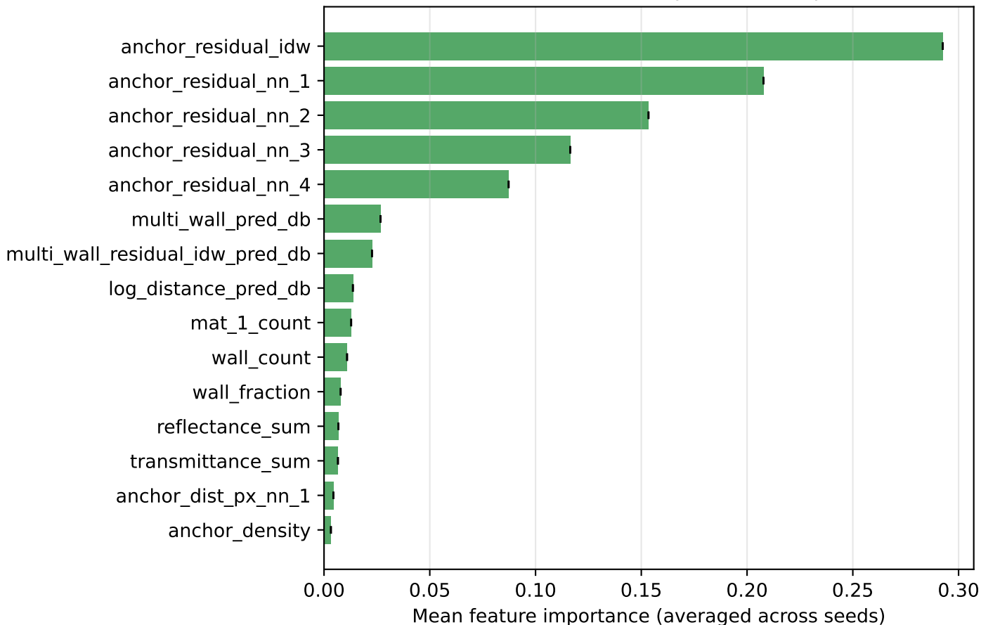
WallPath-PI feature importance (top 15)
