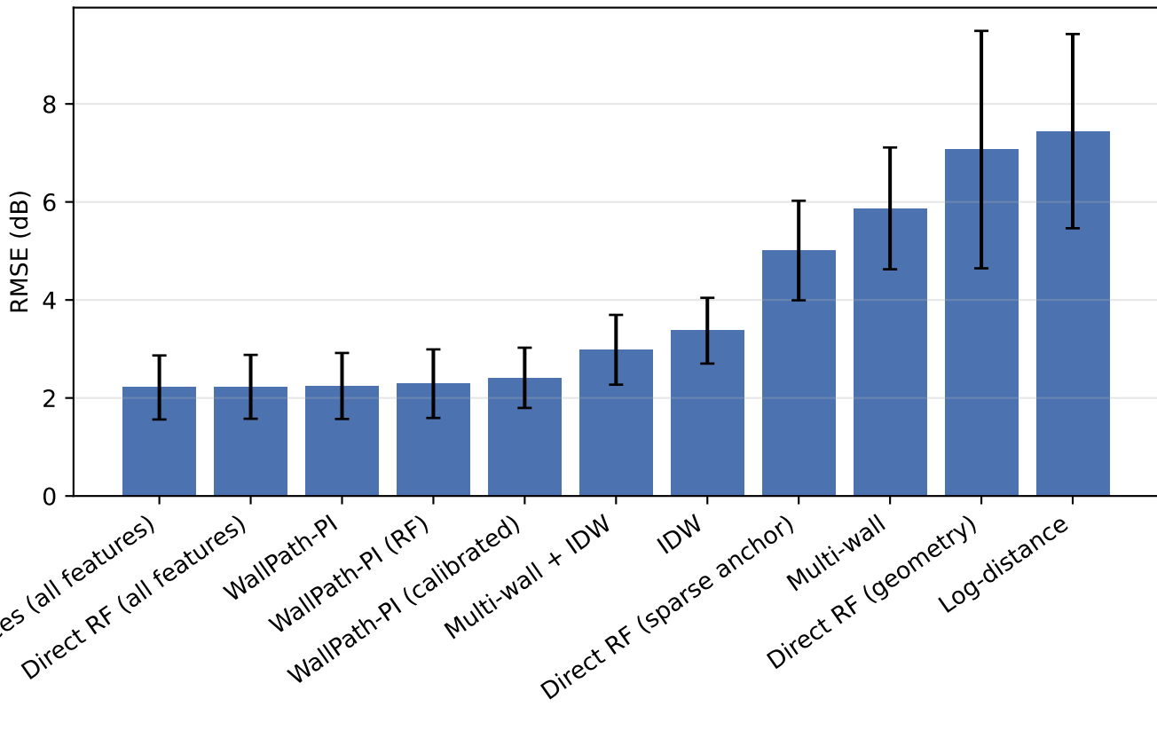
Method comparison at sparse rate 0.05
