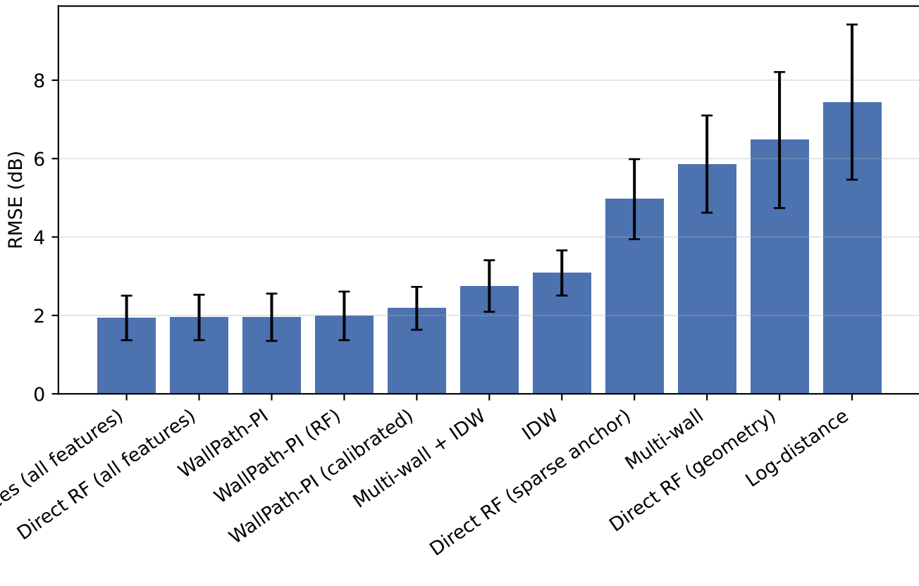
Method comparison at sparse rate 0.1
