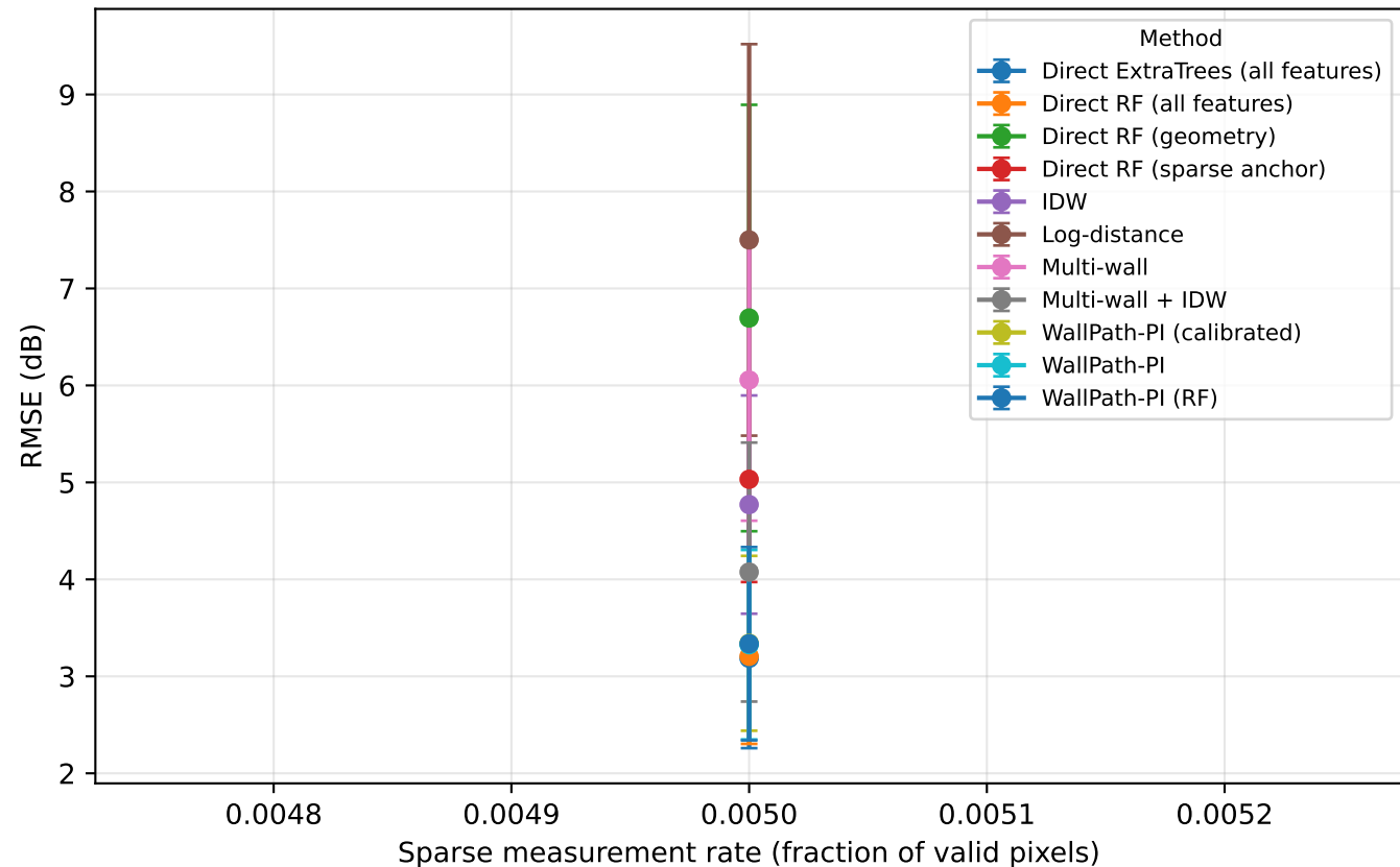
Sparse-budget path-loss reconstruction
