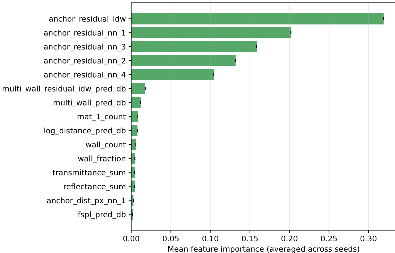
WallPath-PI feature importance (top 15)
