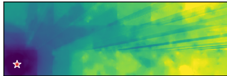
(c) WallPath-PI RMSE = 4.00 dB
