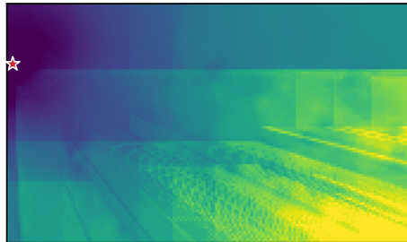
(c) WallPath-PI RMSE = 3.74 dB
