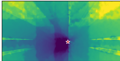
(c) WallPath-PI RMSE = 2.06 dB
