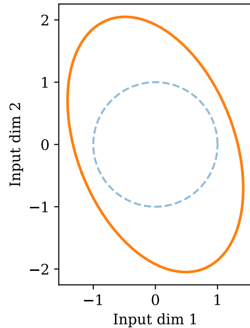
KL/Fisher Metric: J^T D^{-1} J
