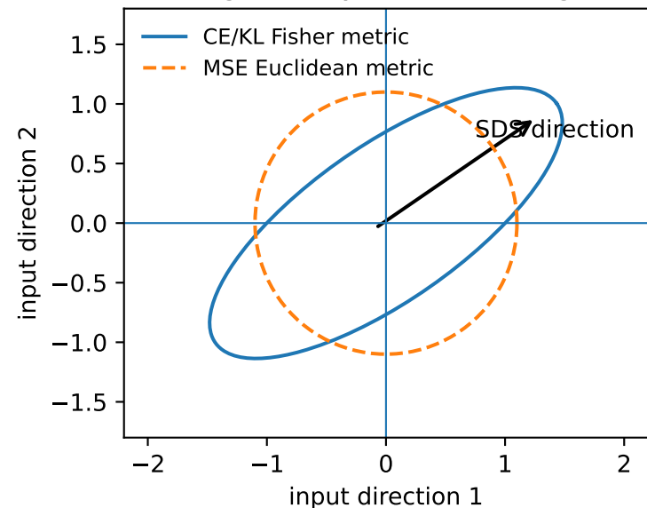
(b) Fisher geometry vs Euclidean geometry
