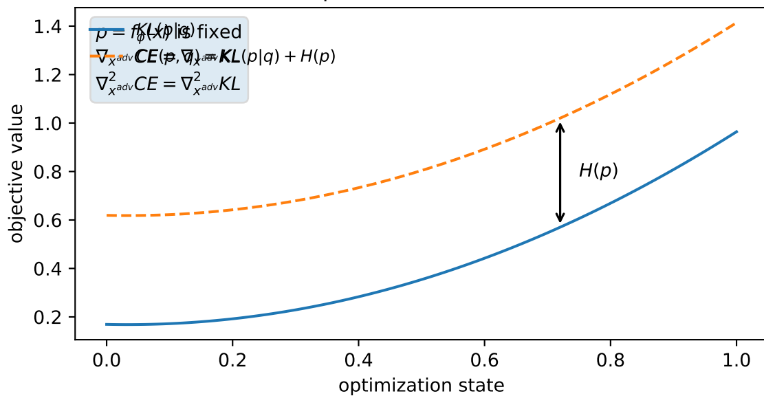
(c) CE-KL equivalence under fixed anchor
