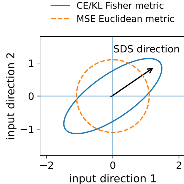
(b) Fisher geometry vs Euclidean geometry
