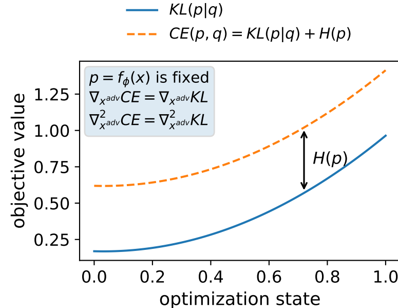
(c) CE-KL equivalence under fixed anchor
