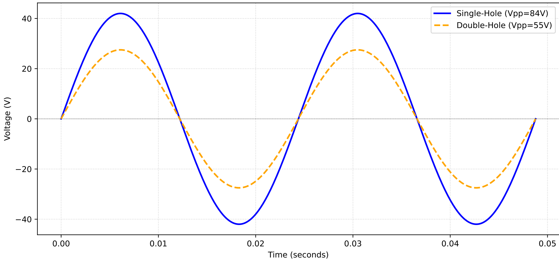
TENS Device Waveform Simulation - Mode 24 (41-25 Hz)
