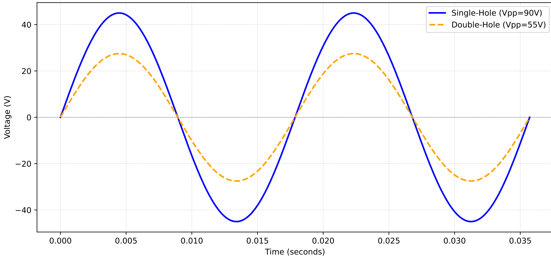
TENS Device Waveform Simulation - Mode 8 (56-22 Hz)
