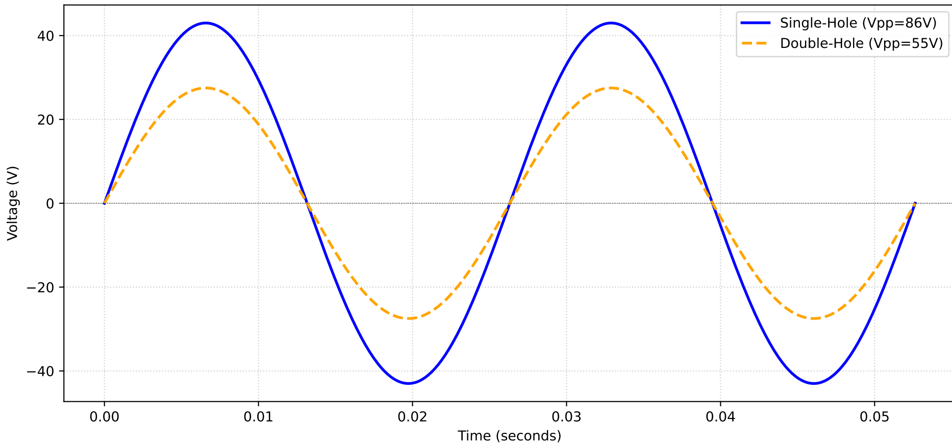
TENS Device Waveform Simulation - Mode 22 (38-22-38 Hz)
