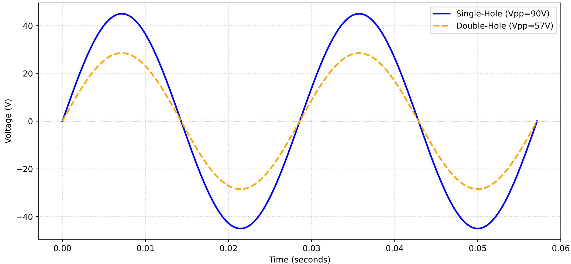
TENS Device Waveform Simulation - Mode 4 (35-22-35 Hz)
