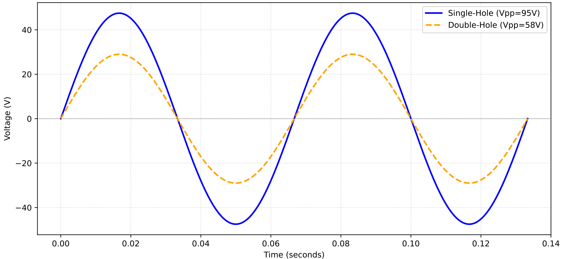
TENS Device Waveform Simulation - Mode 1 (15 Hz)
