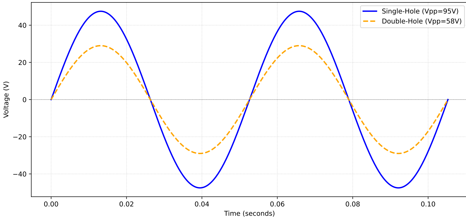
TENS Device Waveform Simulation - Mode 6 (3-19 Hz)
