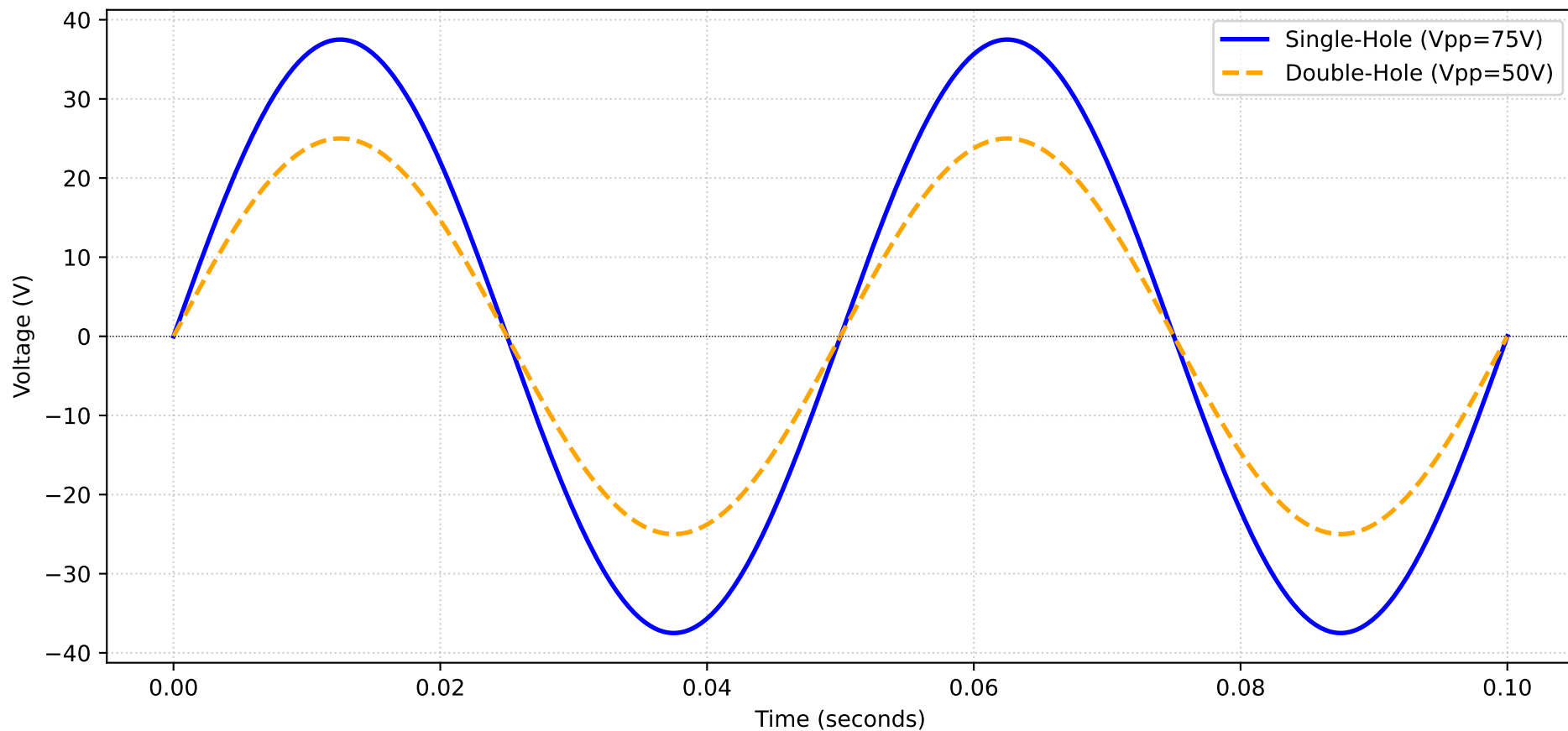
TENS Device Waveform Simulation - Mode 19 (20 Hz)
