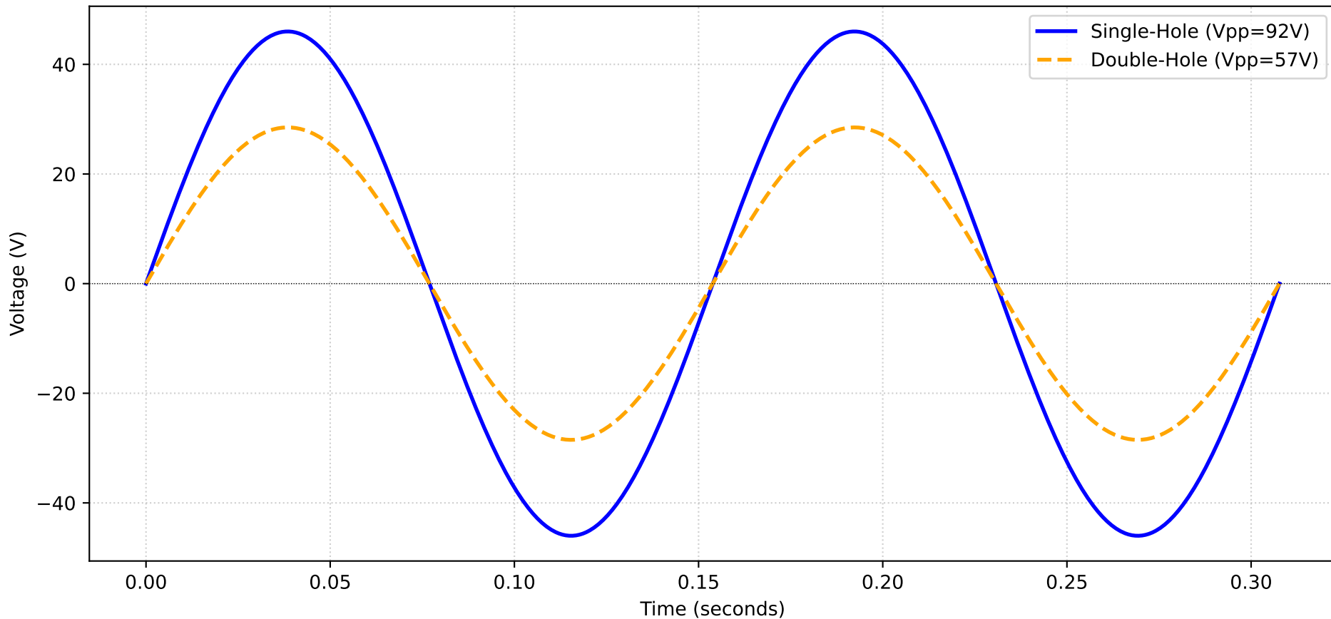
TENS Device Waveform Simulation - Mode 17 (6.5 Hz)
