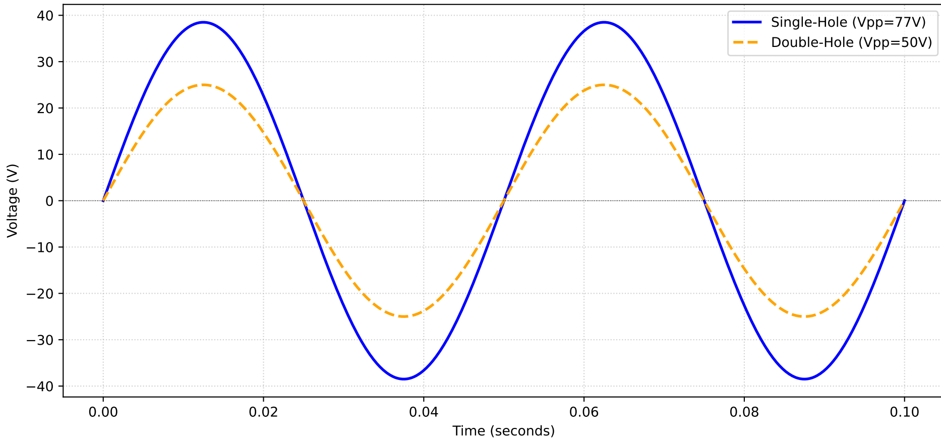
TENS Device Waveform Simulation - Mode 21 (20 Hz)
