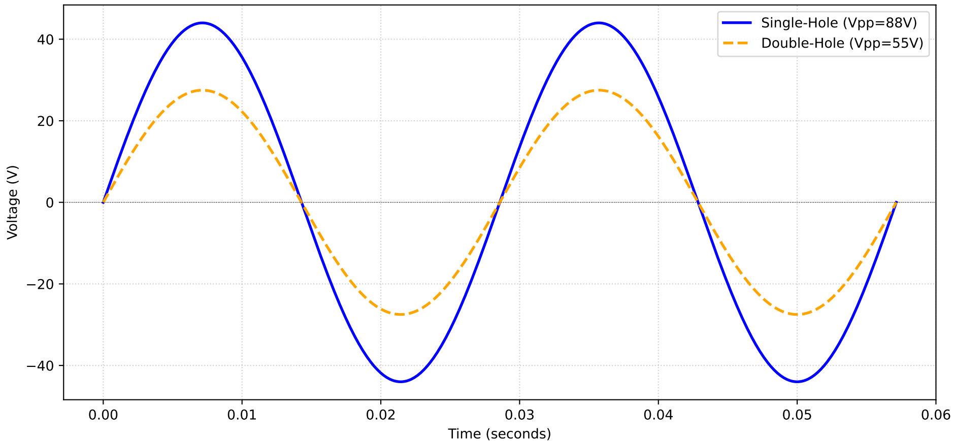
TENS Device Waveform Simulation - Mode 14 (35-22-35 Hz)
