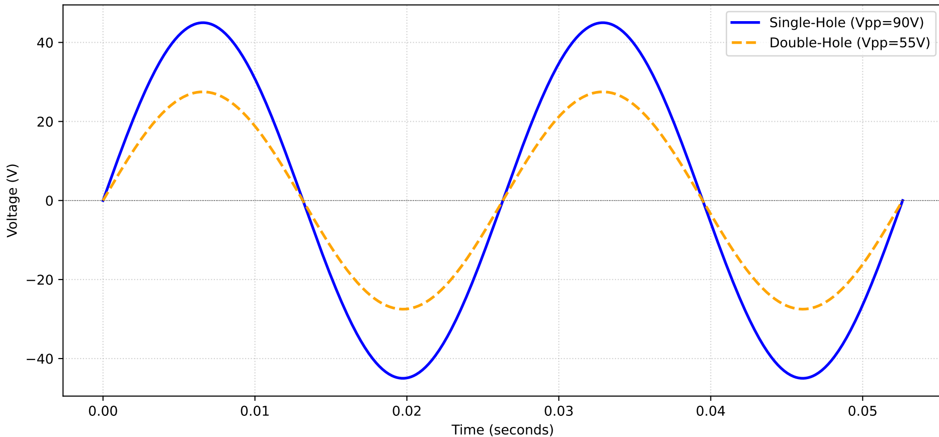
TENS Device Waveform Simulation - Mode 10 (38-24-38 Hz)
