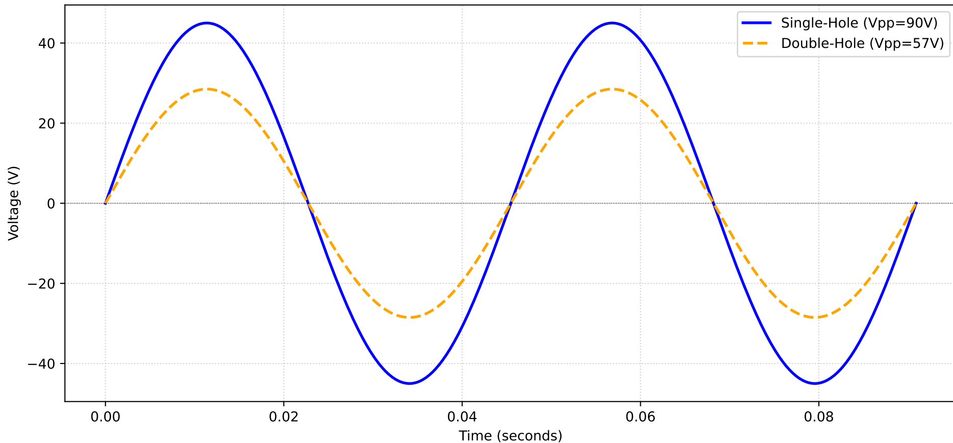
TENS Device Waveform Simulation - Mode 20 (3-22 Hz)
