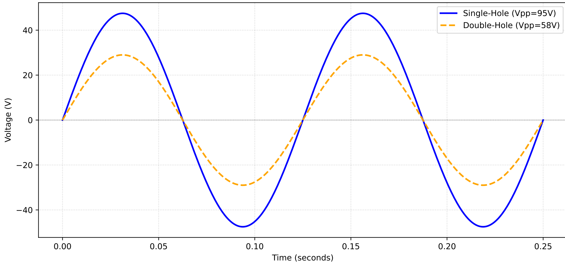
TENS Device Waveform Simulation - Mode 7 (8 Hz)
