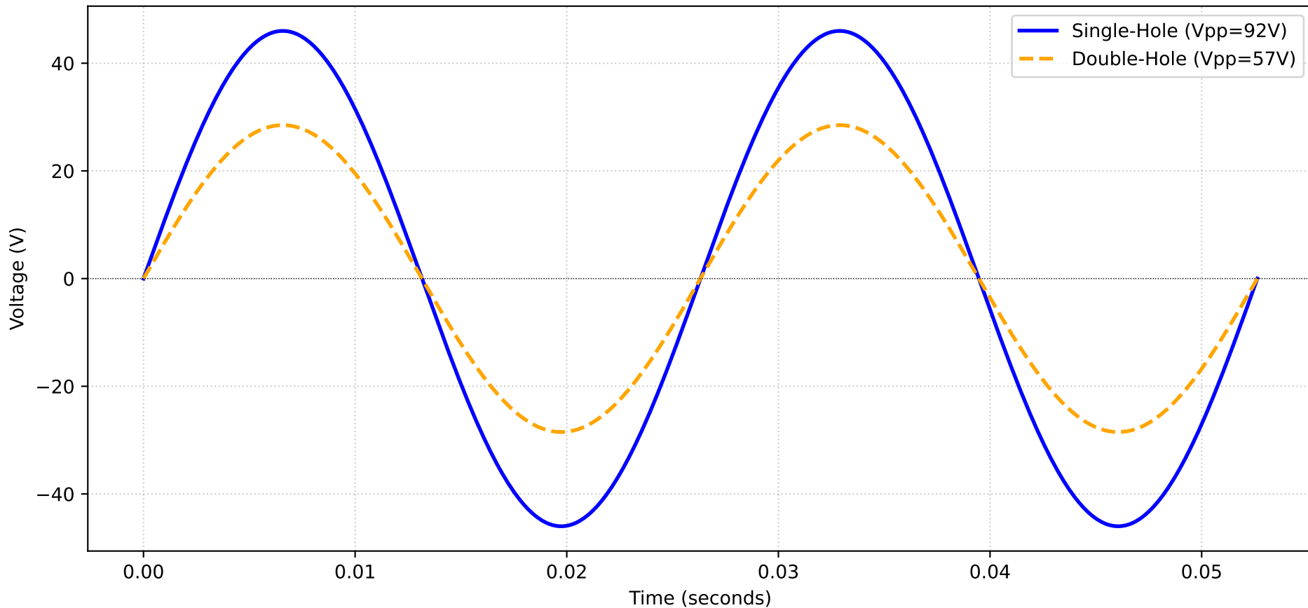
TENS Device Waveform Simulation - Mode 3 (38-22-38 Hz)
