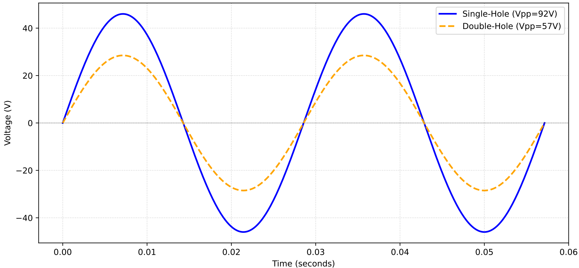
TENS Device Waveform Simulation - Mode 11 (35-22-35 Hz)
