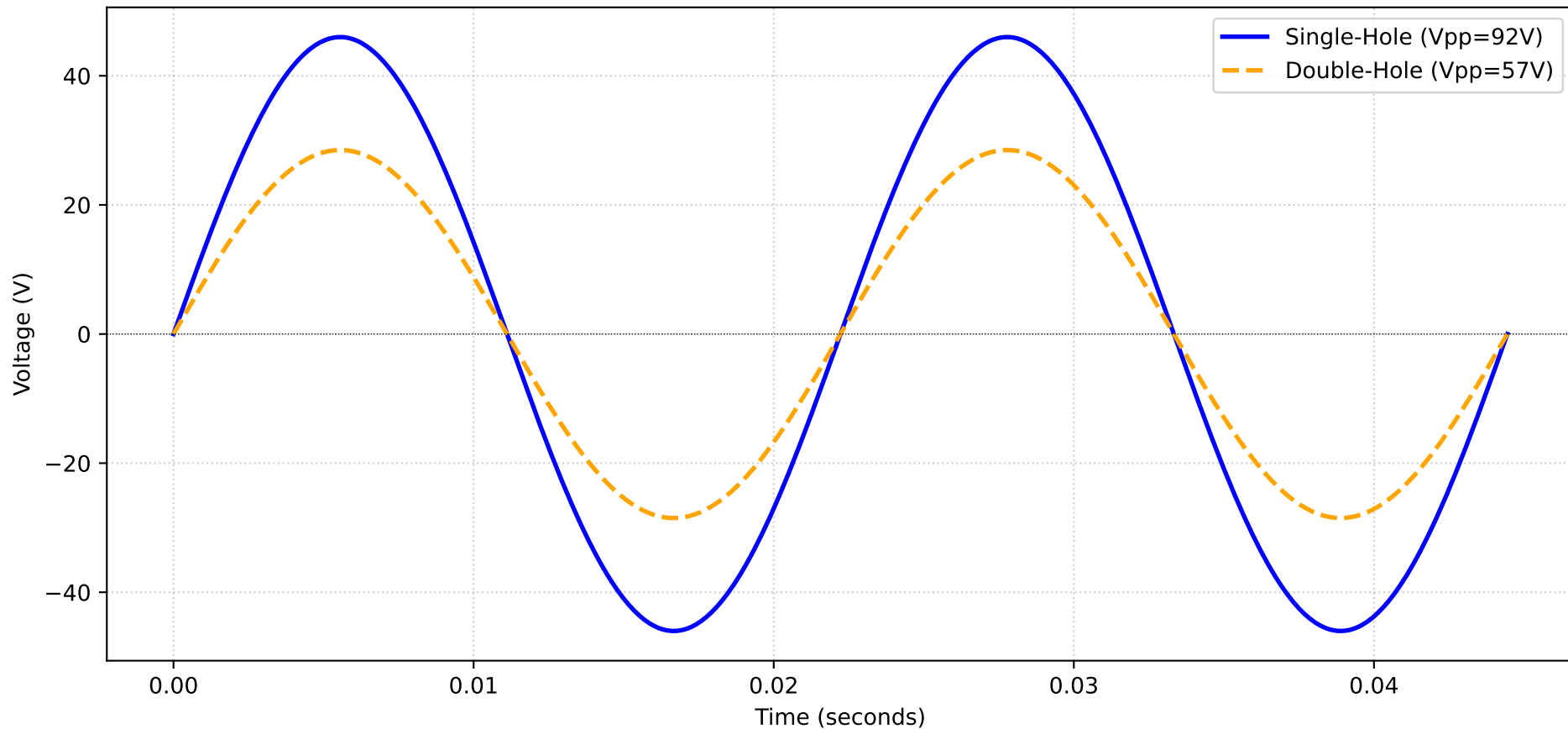
TENS Device Waveform Simulation - Mode 12 (45-22 Hz)
