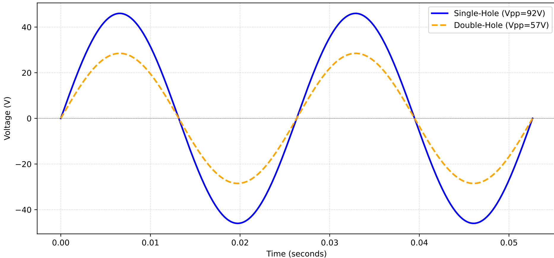
TENS Device Waveform Simulation - Mode 2 (38 Hz)
