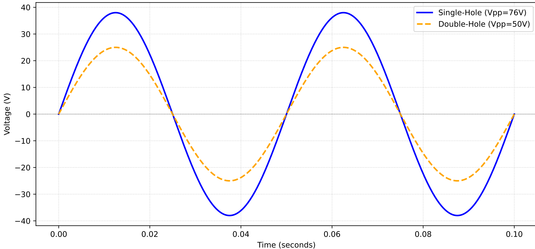
TENS Device Waveform Simulation - Mode 23 (20 Hz)
