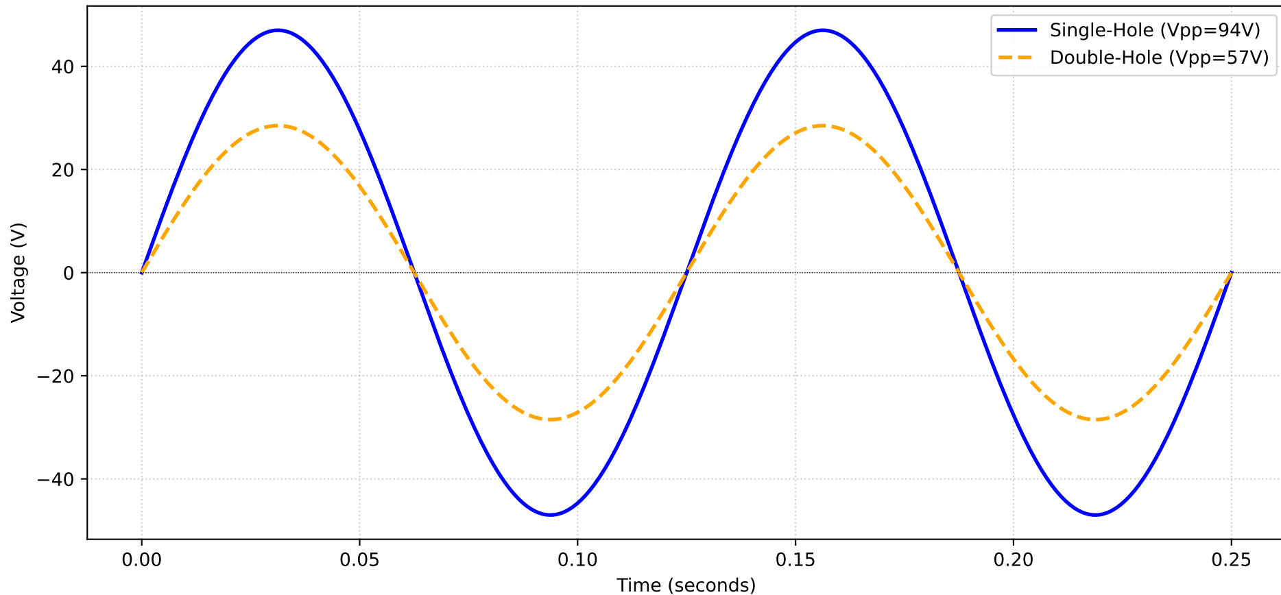
TENS Device Waveform Simulation - Mode 9 (8 Hz)
