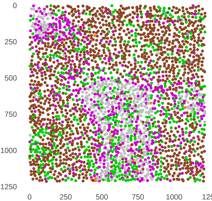
mIF sample 10068868 ROI 005
