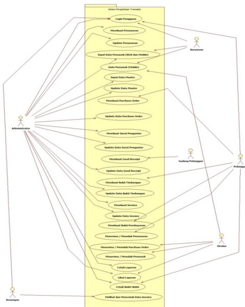
Gambar 4. Use-Case Diagram
