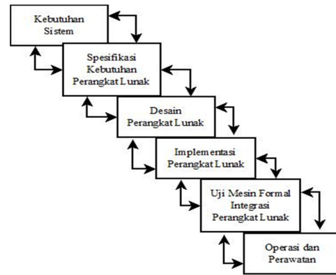
Gambar 1. Metode Waterfall [10]
