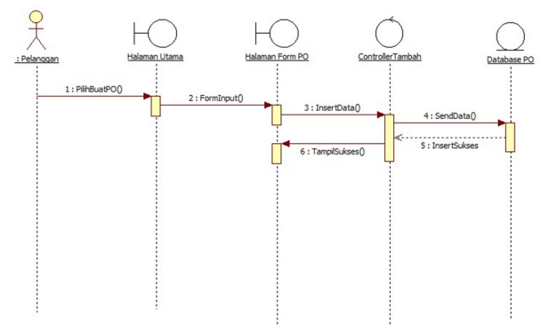
Gambar 5. Sequece Diagram Input Data Pembelian/ Purchase Order
