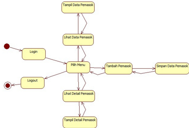
Gambar 8. StateChart Diagram
