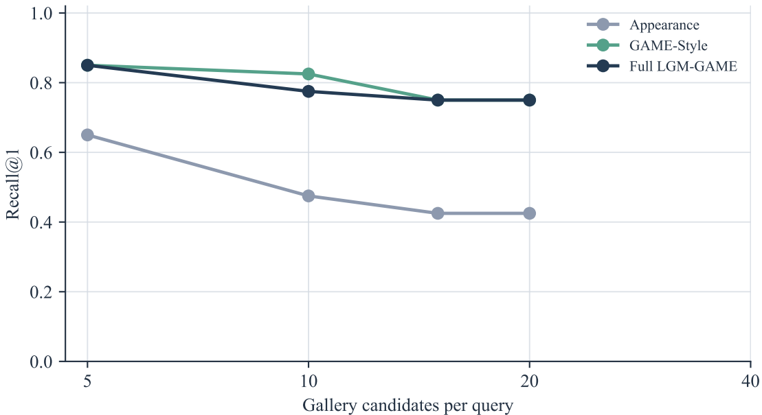
Candidate-scale stress test
