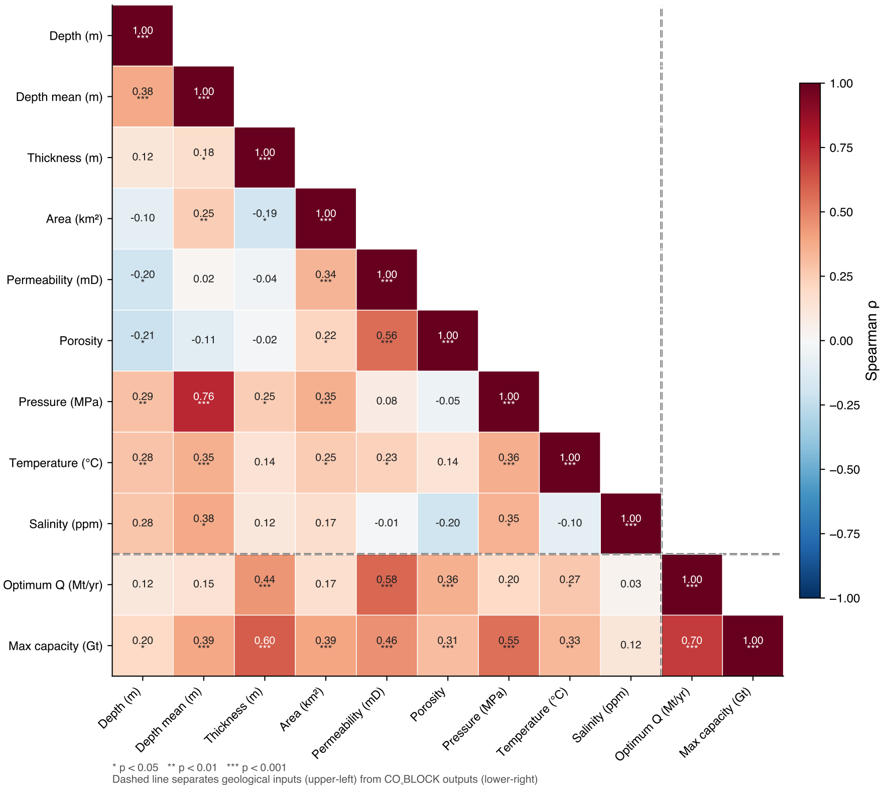
Figure 2 | Geological parameter correlation (Spearman \rho , t = 150 yr)
