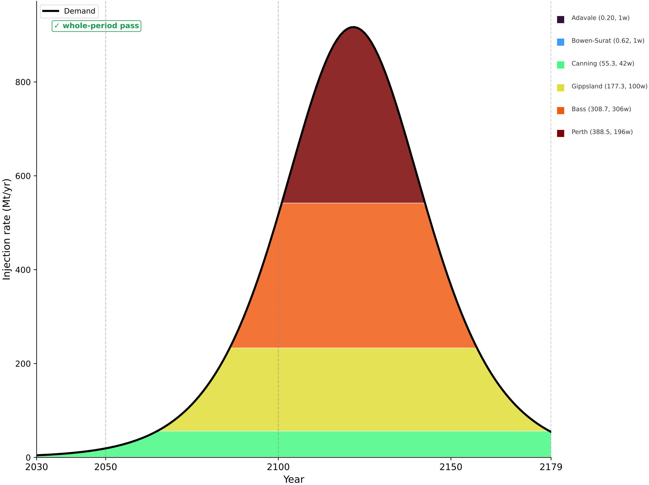
Logistic
