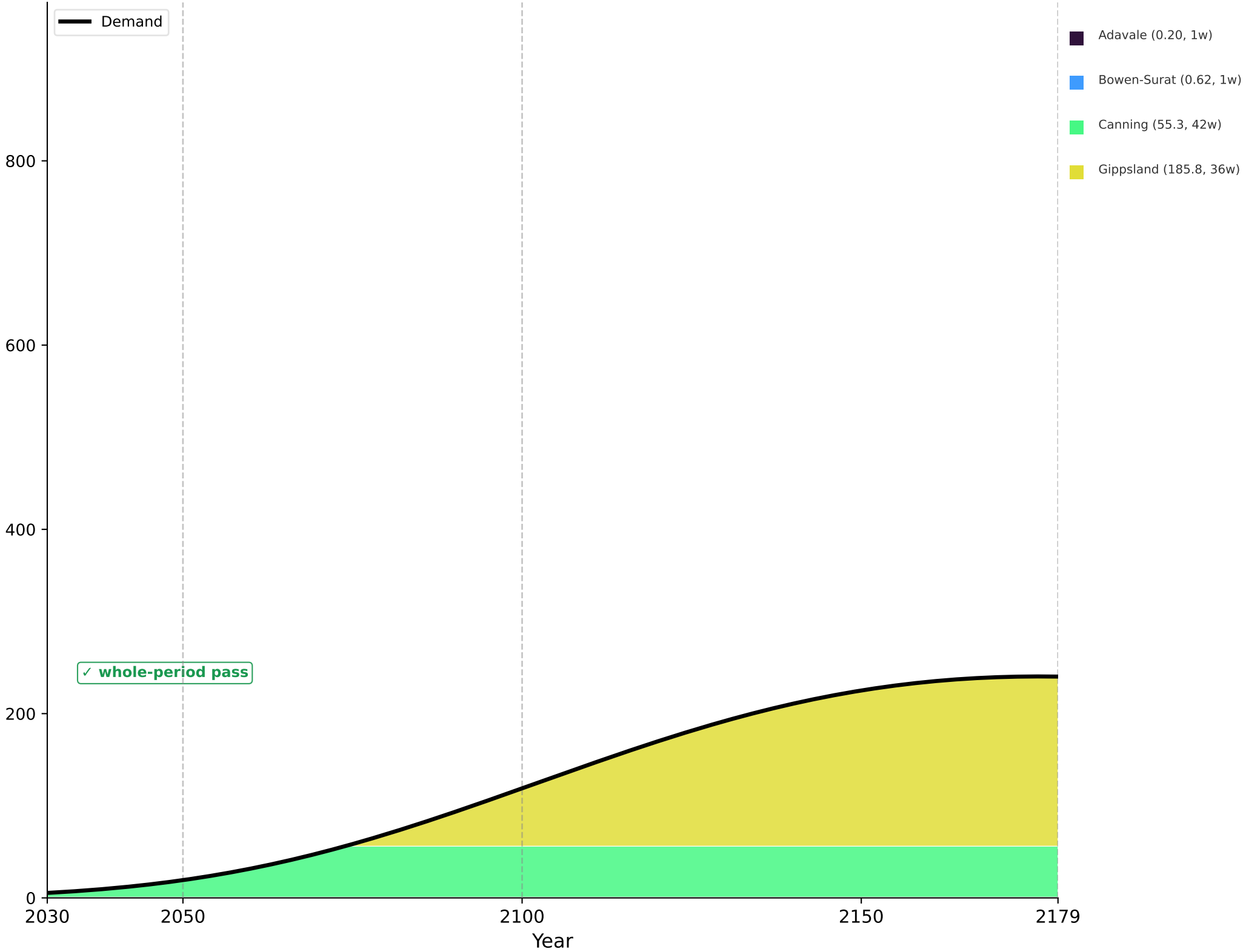
Gompertz
