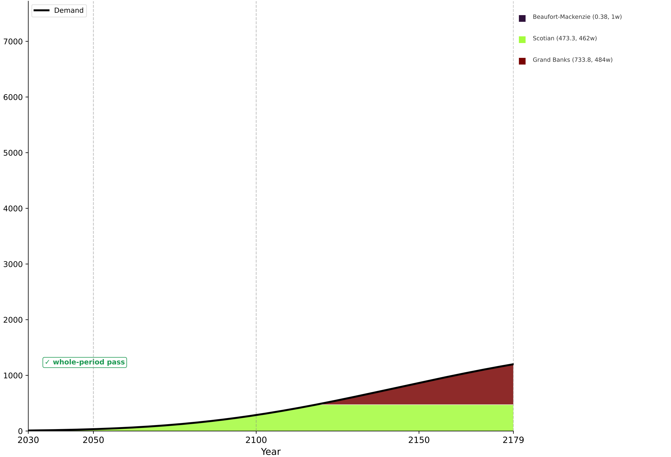
Gompertz
