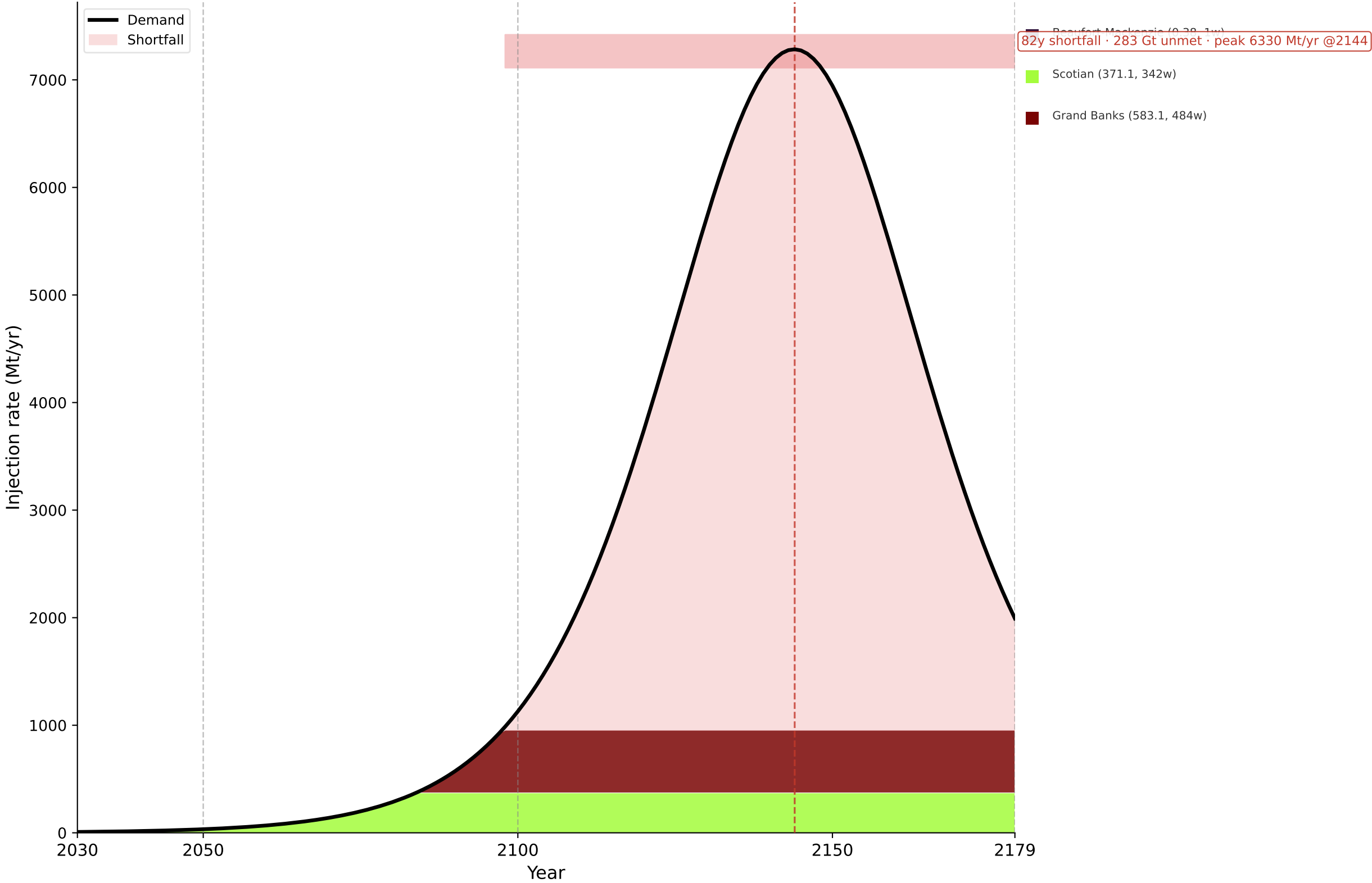
Logistic
