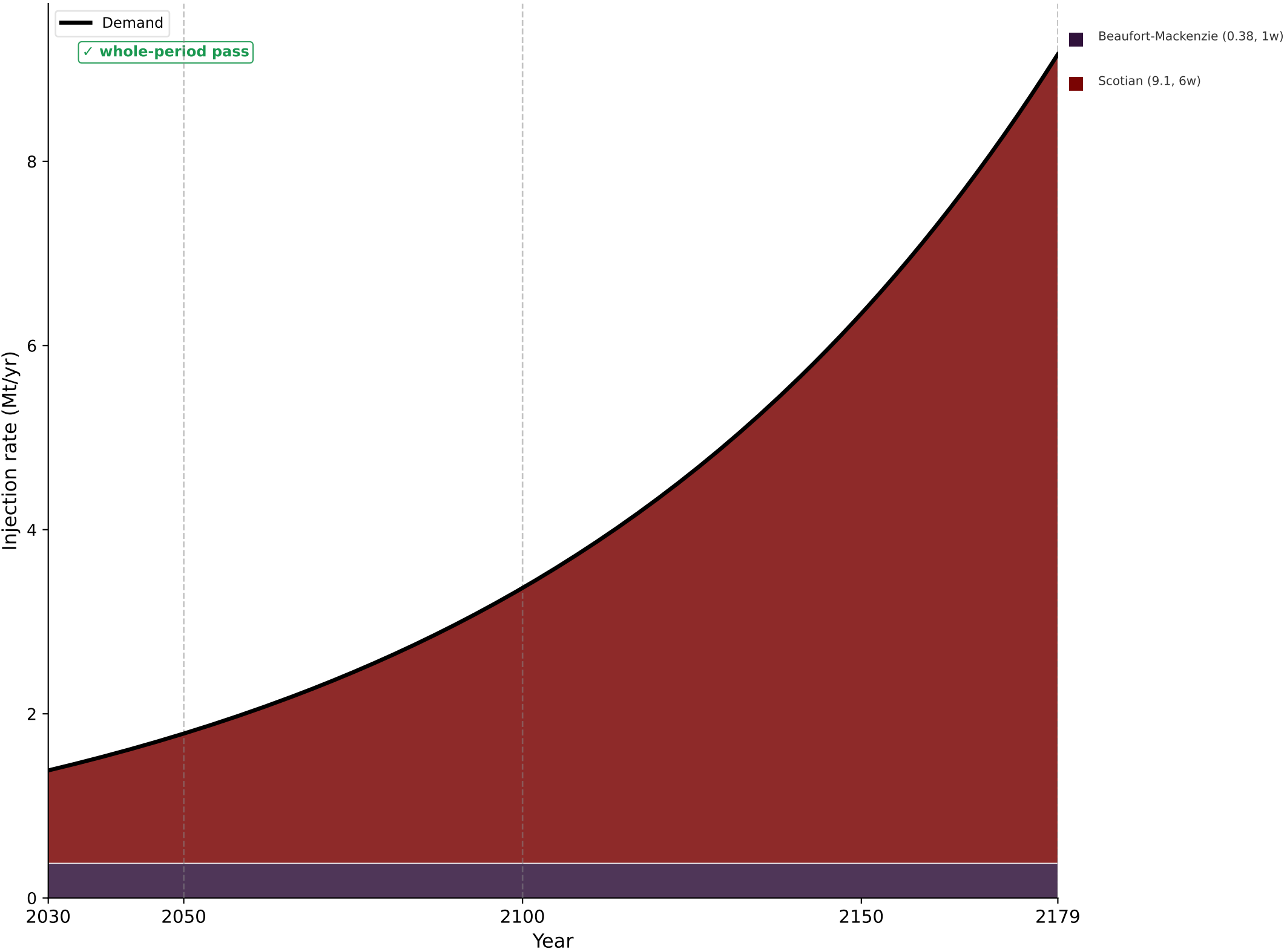
Logistic
