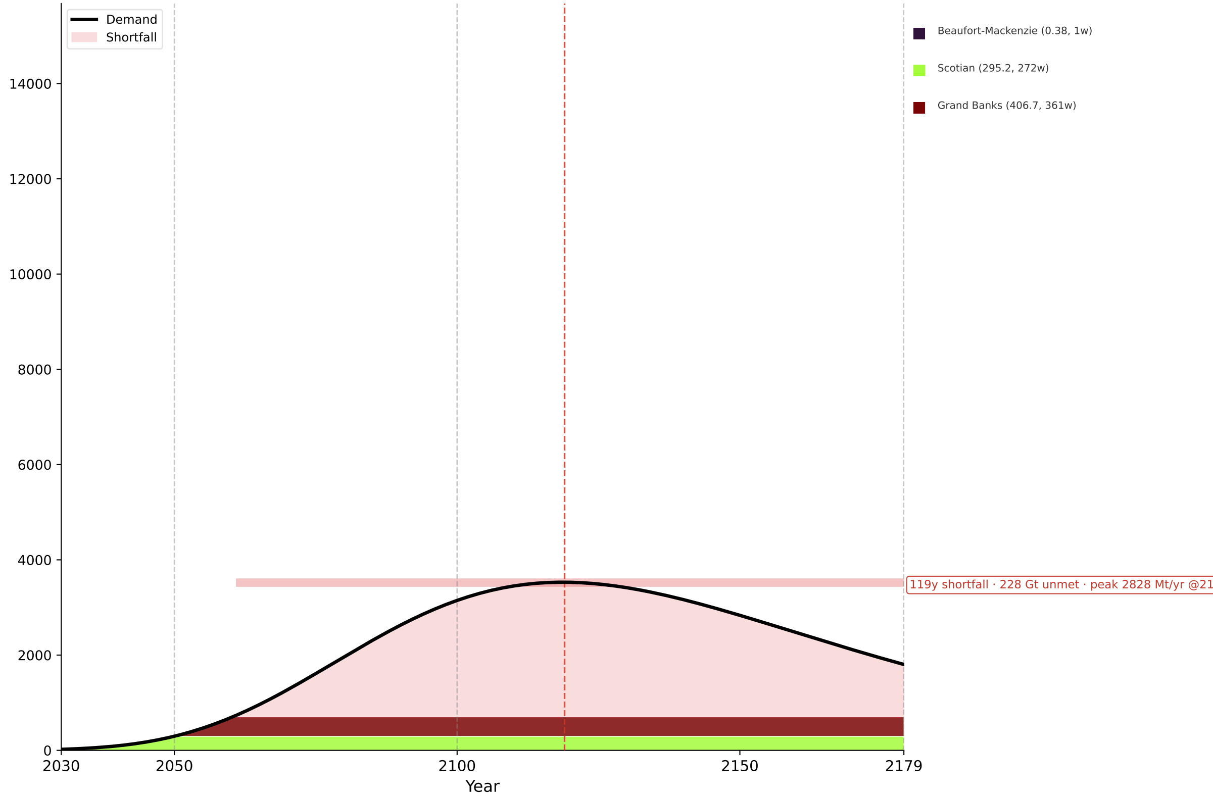
Gompertz
