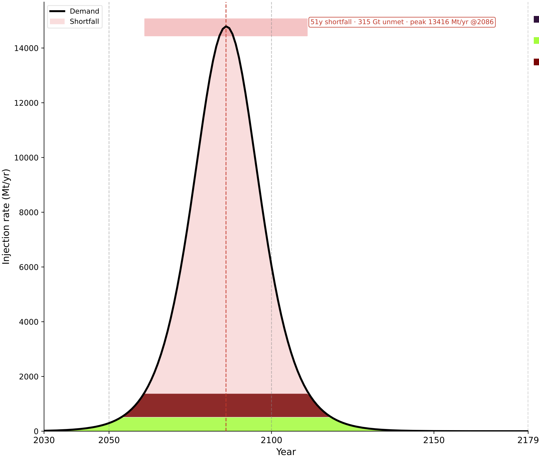
Logistic
