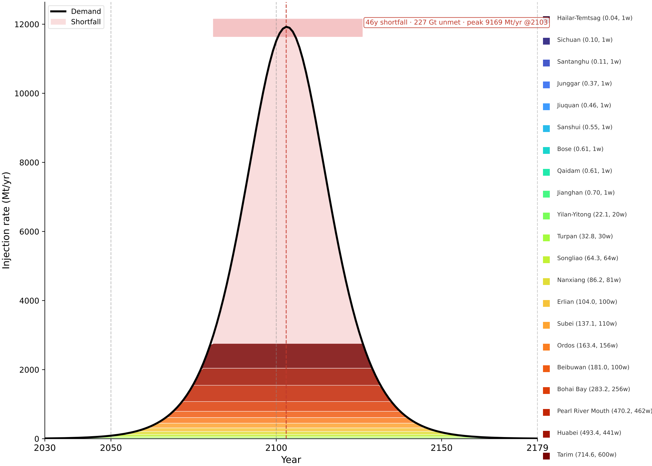
Logistic
