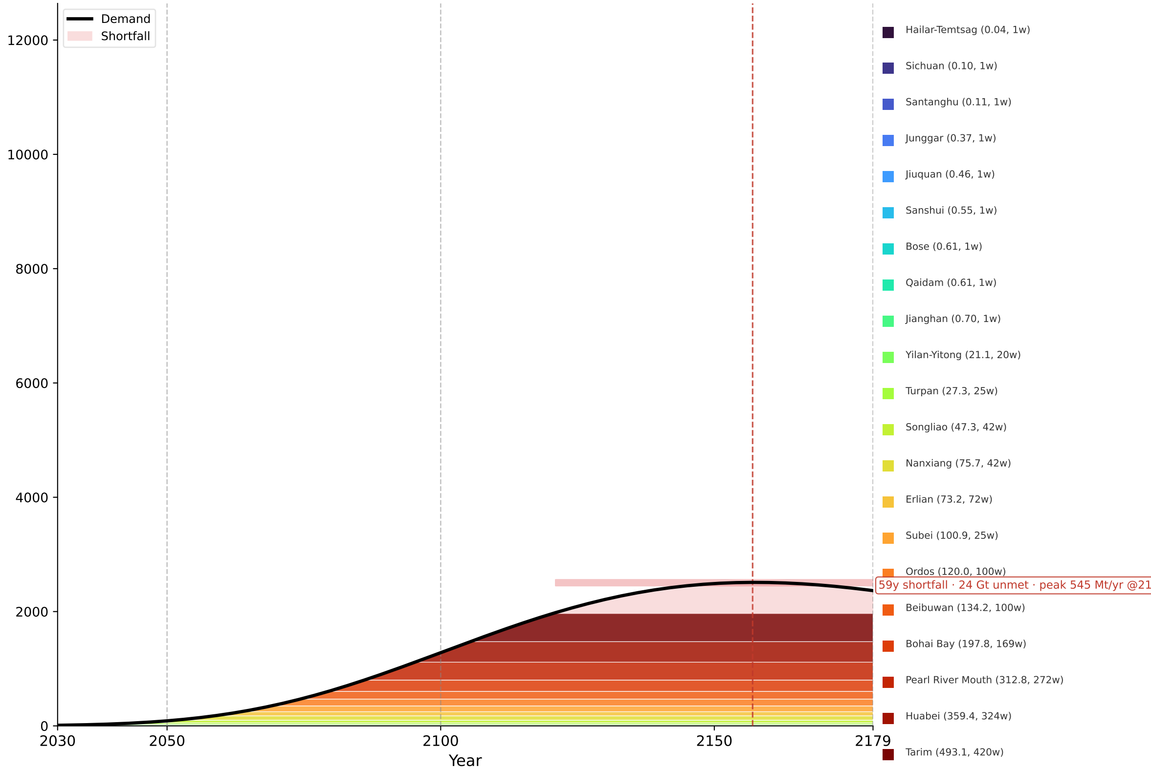
Gompertz
