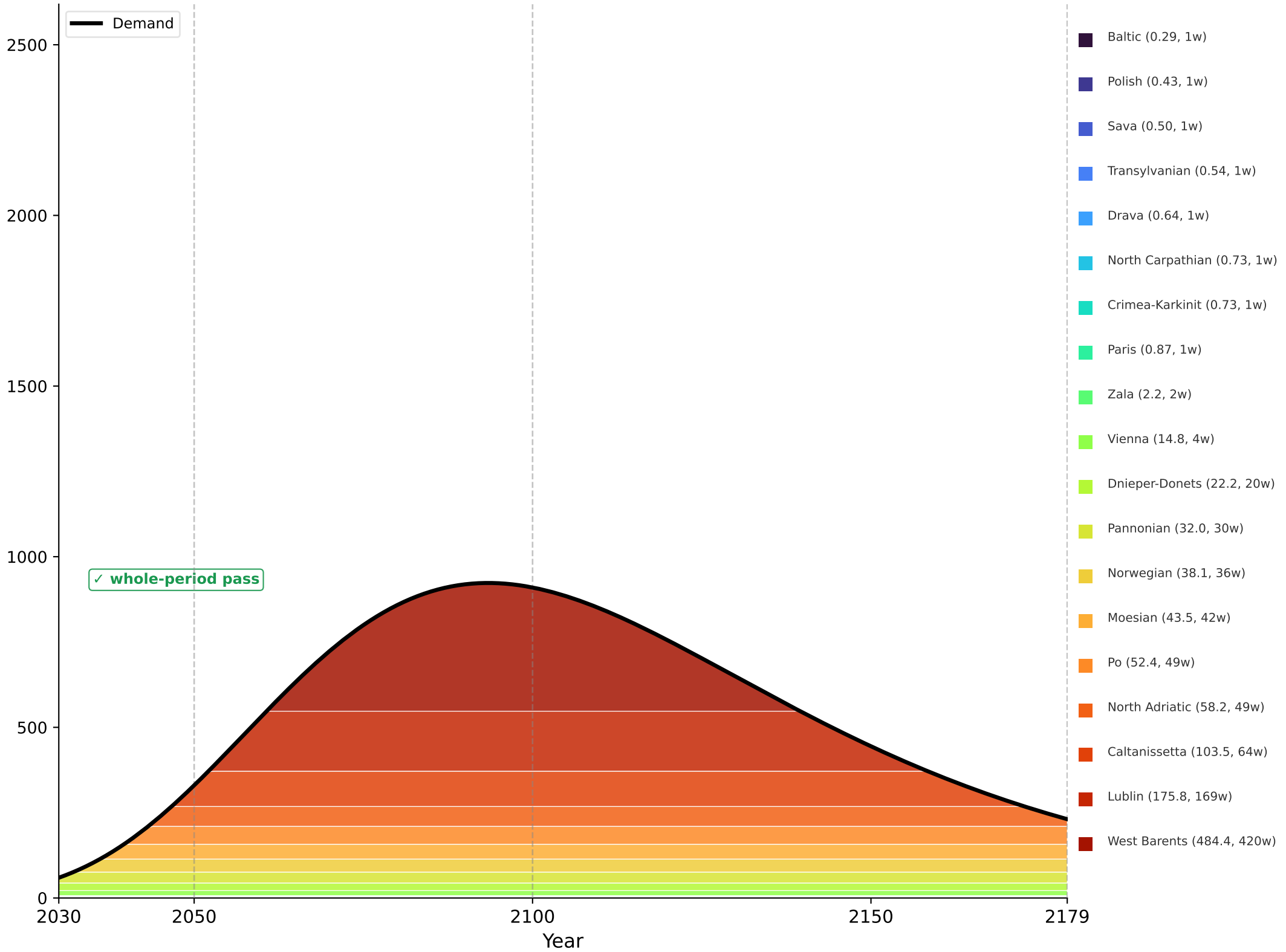
Gompertz
