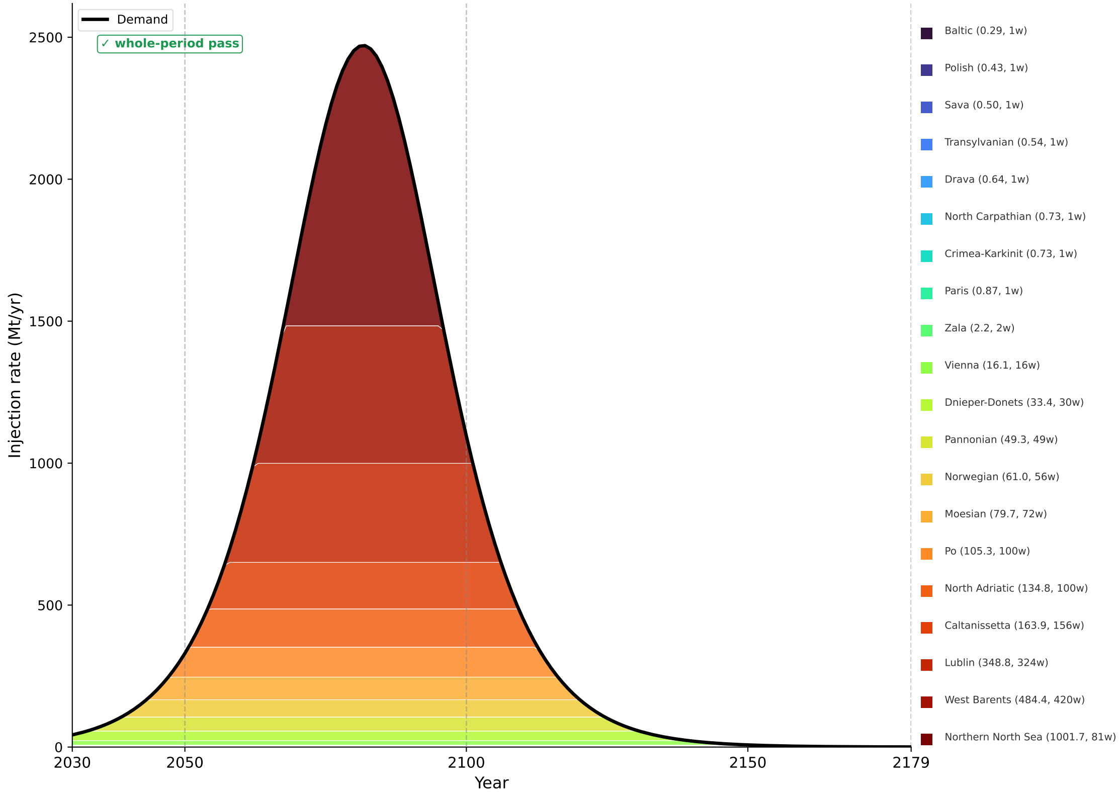
Logistic
