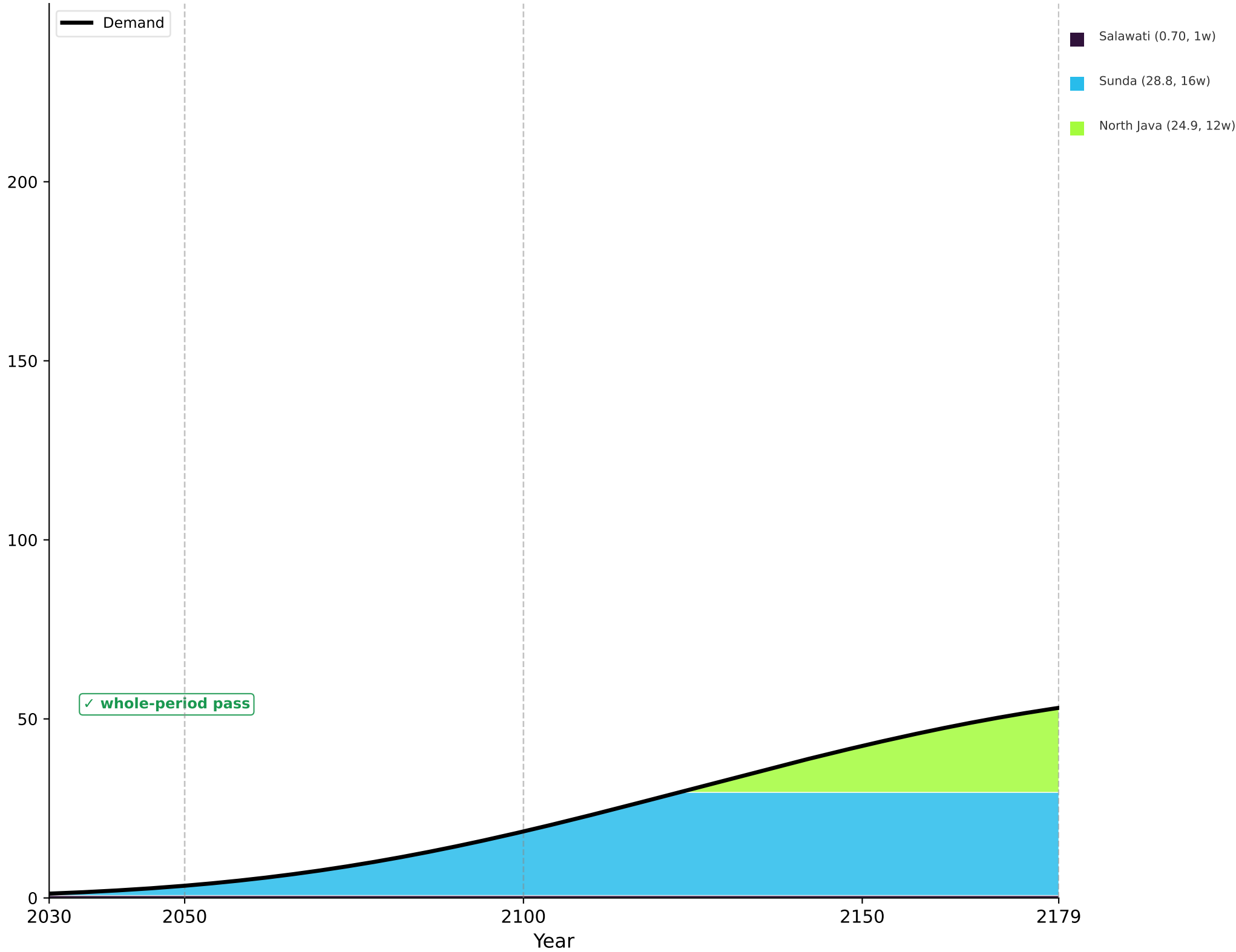
Gompertz
